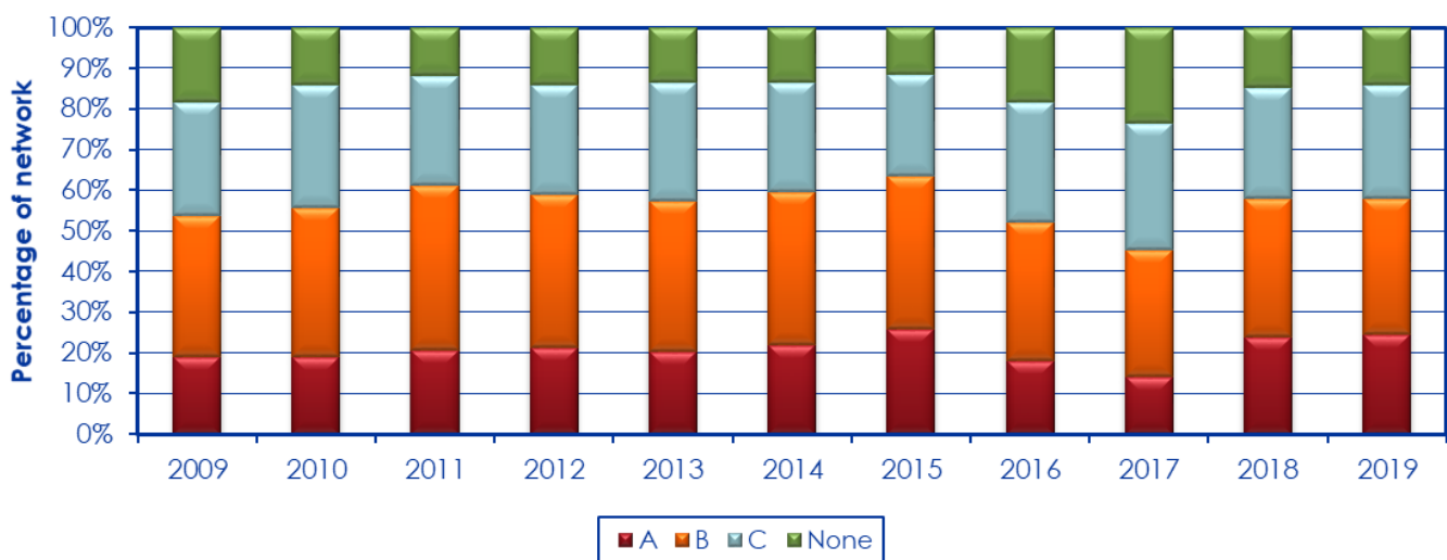
Figure 4-56: Resealing demand of paved roads according to urgency 2009 to 2019 (includes UniCity roads)
