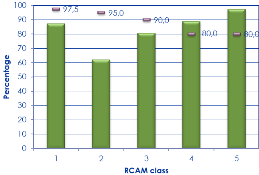
Figure 4-37: High texture exposure per RCAM class compared with preliminary LOS targets in 2018
