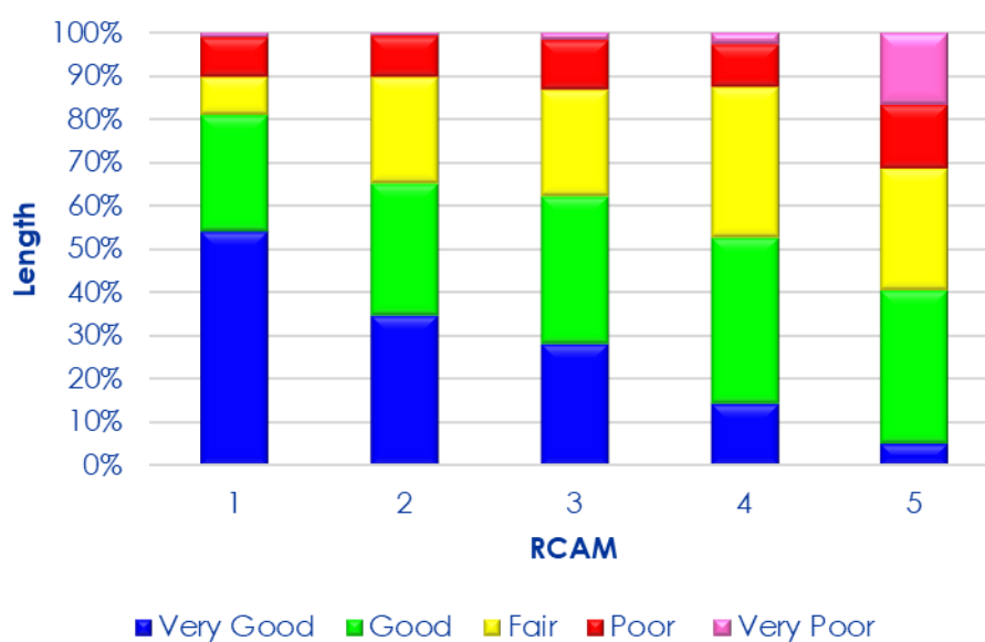
Figure 4-8: Condition distribution per kilometre by RCAM Class for paved roads as at December 2019 including UniCity roads
