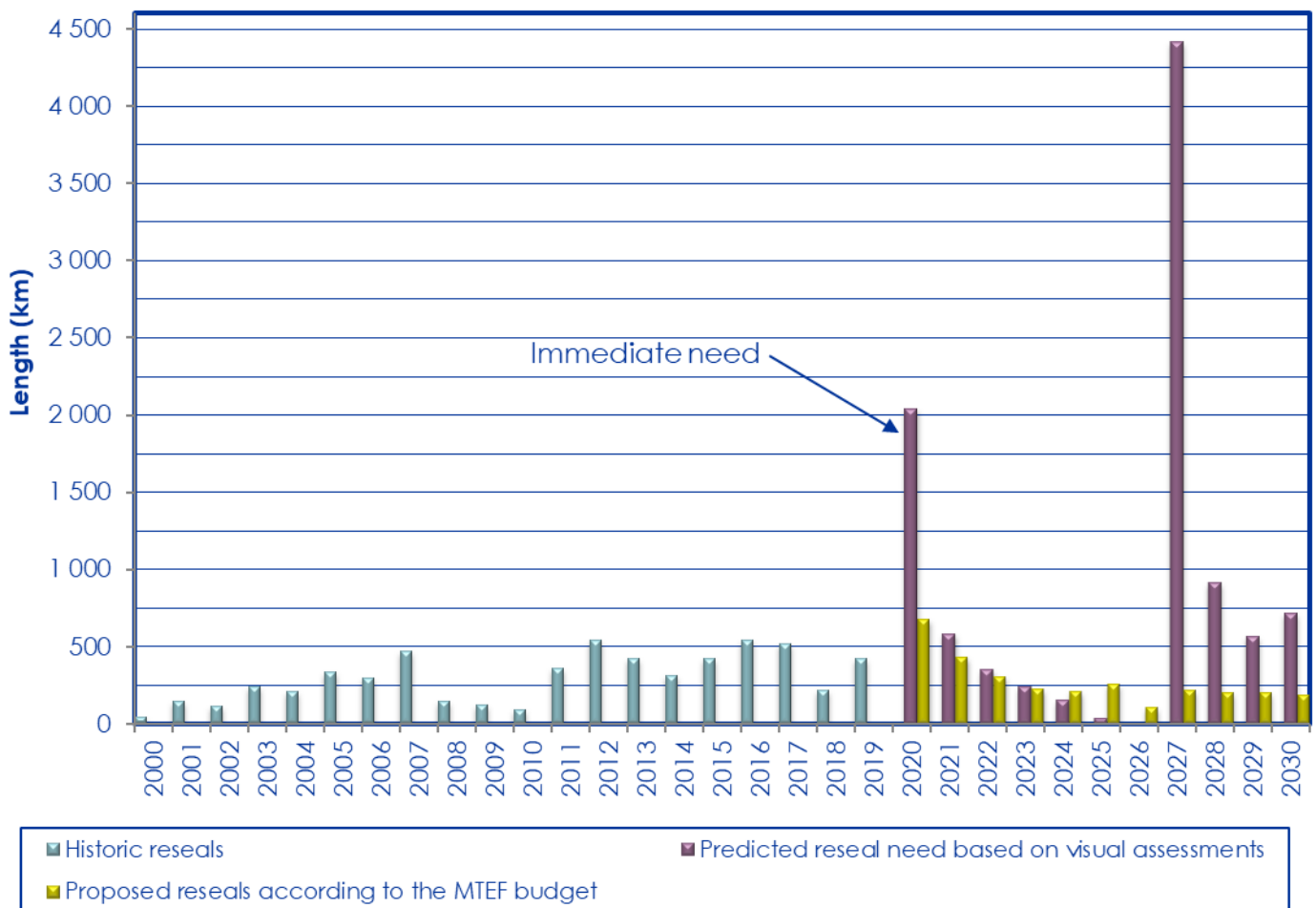
Figure 5-1: Historic resealing of paved roads versus the predicted need and proposed MTEF budget resealing programme from 2000 to 2030
