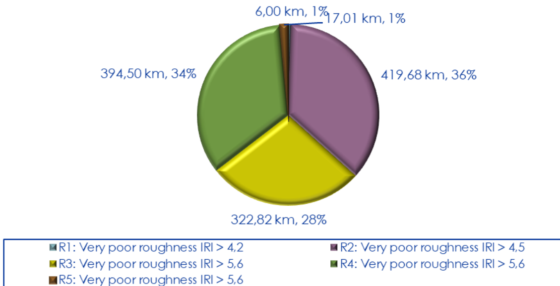
Figure 5-7: Distribution of very poor paved roads according to roughness values in 2016 based on the 2019 length
