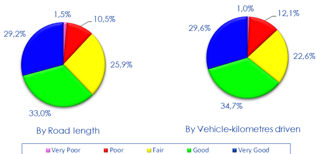
Figure 4-5: Distribution of the VCI of paved roads by road length and vehicle-km as at December 2019 including UniCity roads
