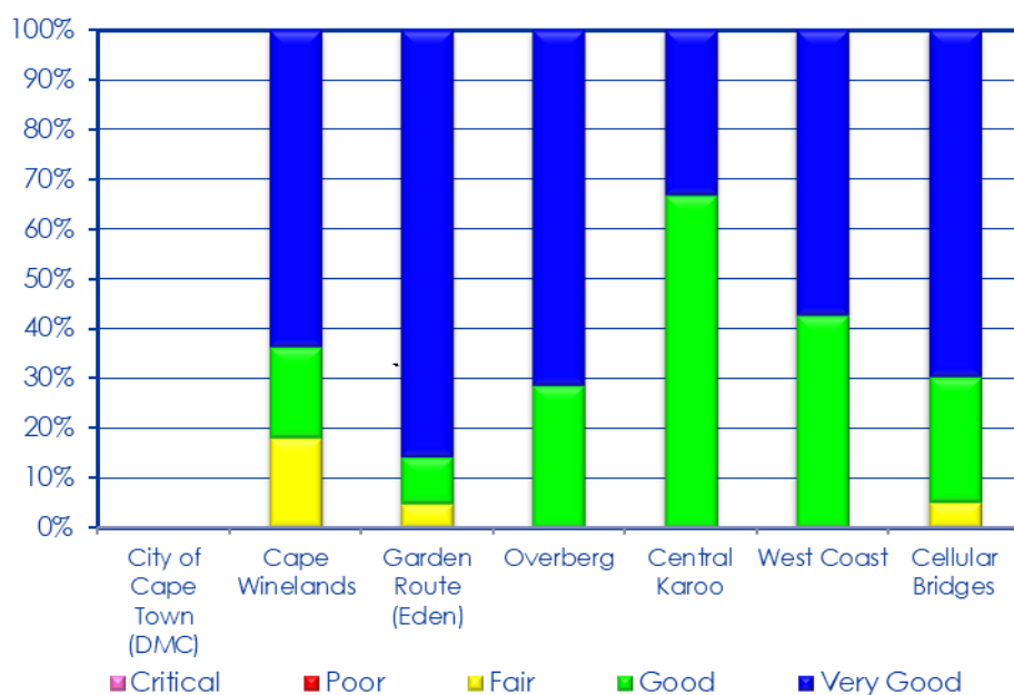
Figure 4-17: ACI for cellular bridges per DM (March 2020)
