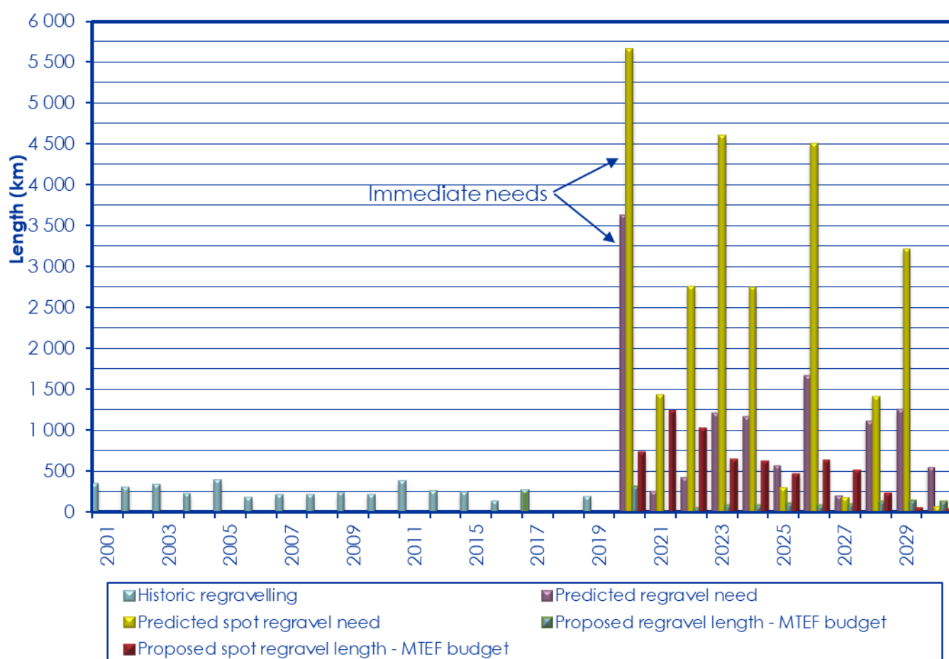
Figure 5-9: Historic regravelling of maintained unpaved roads versus immediate need and proposed intervention of the MTEF budget for 2001 to 2030
