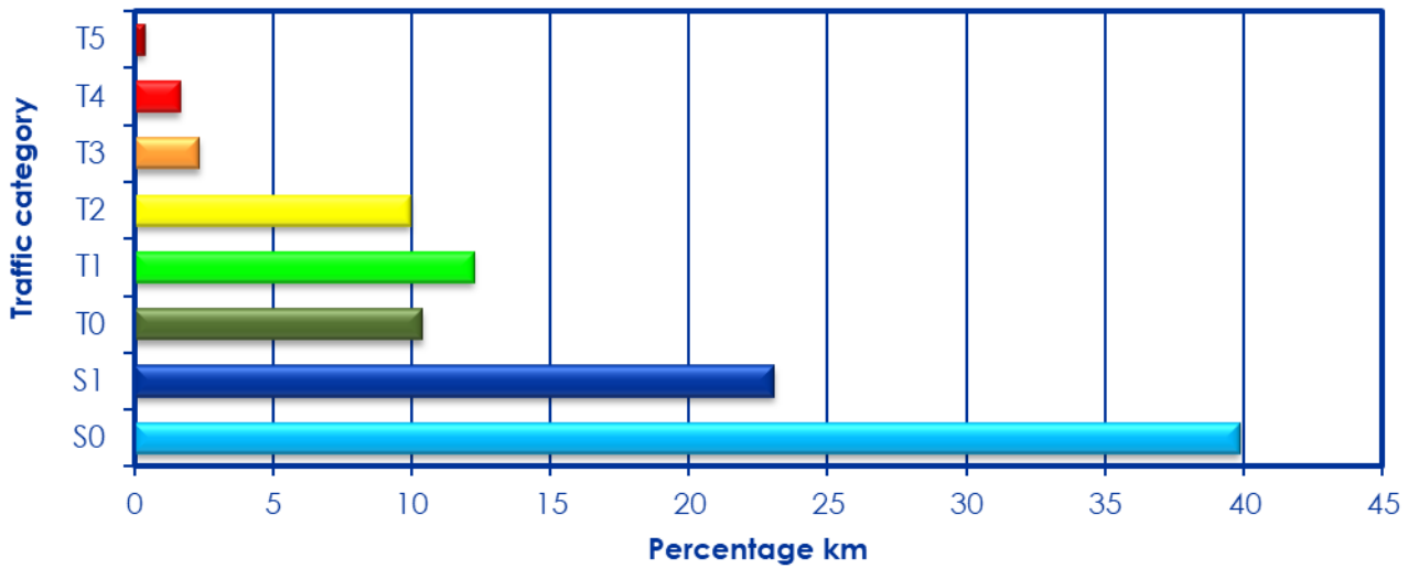
Figure 4-3: Traffic categories and their percentage of km of the network for 2020 (excluding UniCity roads)
