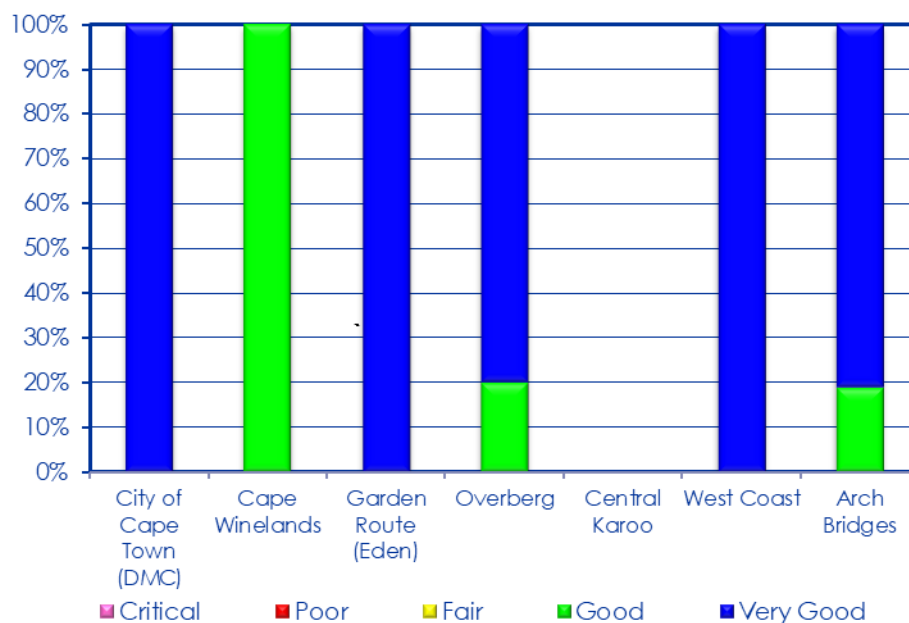
Figure 4-16: ACI for arch bridges per DM (March 2020)
