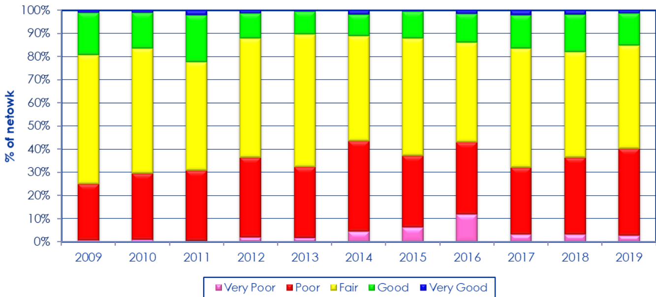
Figure 4-51: Change in the visual condition by road length of maintained unpaved road network 2009 to 2019
