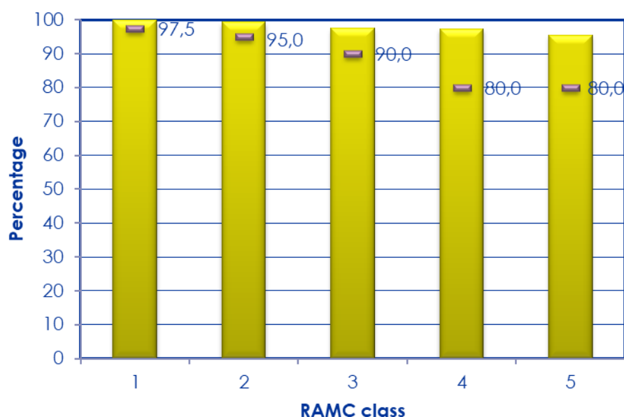
Figure 4-36: Low rut exposure per RCAM class compared with preliminary LOS targets for 2018
