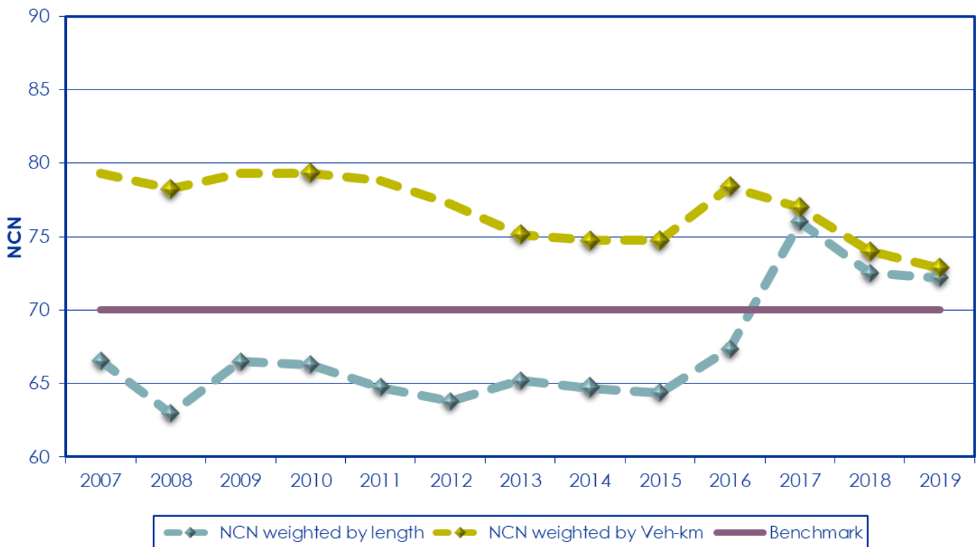
Figure 4-50: The historic trend in the overall network condition of the paved road network 2007 to 2019
