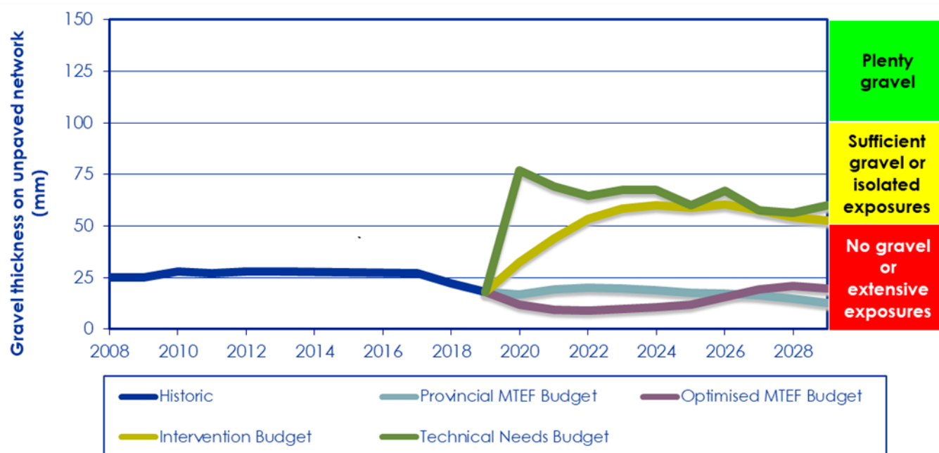
Figure 5-28: Average gravel thickness of maintained unpaved roads
