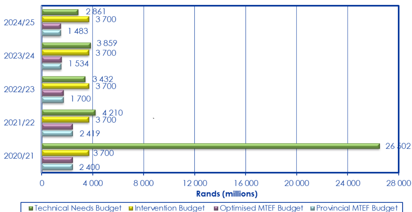
Figure 5-21: Predicted expenditure for regravelling, resealing, light rehabilitation, rehabilitation and upgrading of unpaved roads to paved standards for the four budgets
