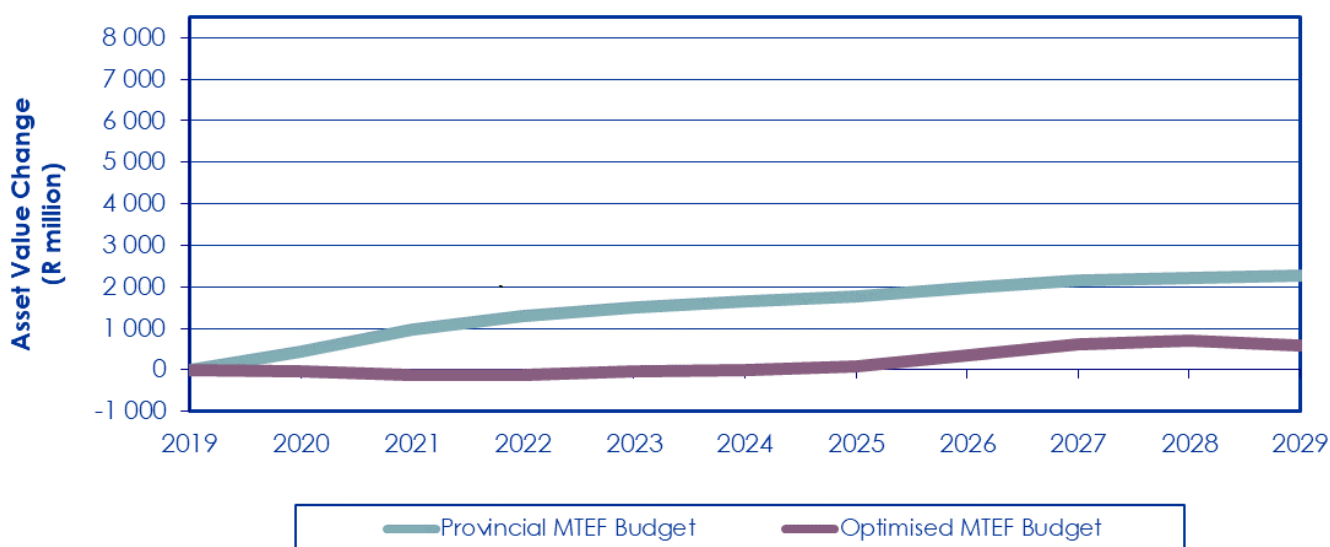
Figure 5-35: Change in asset value of unpaved roads
