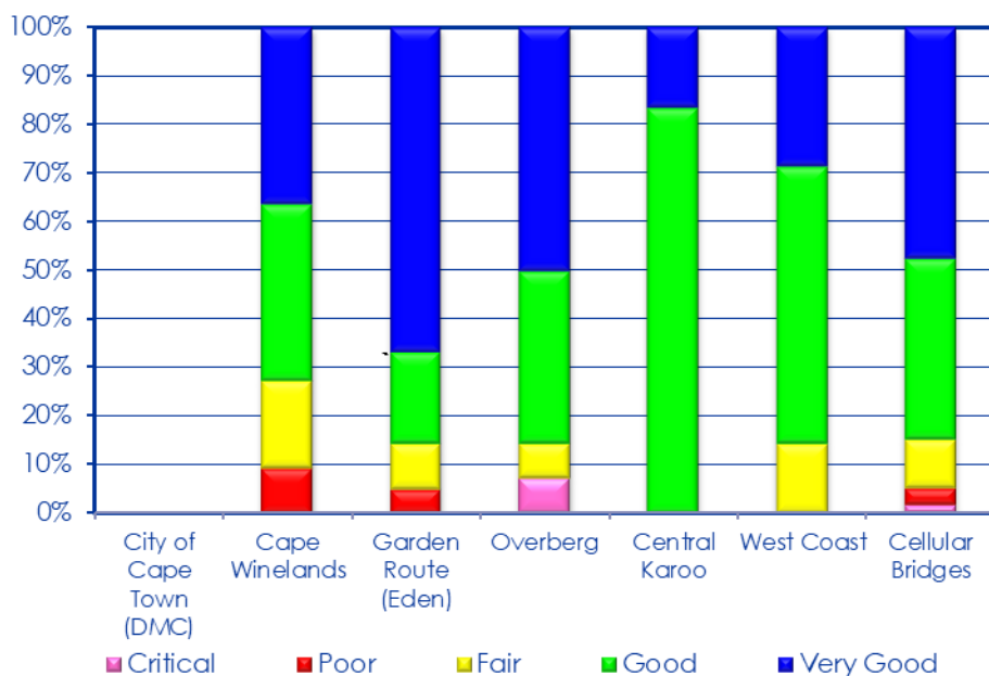
Figure 4-23: PCI for cellular bridges per DM (March 2020)
