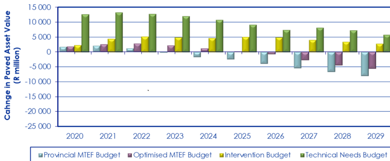
Figure 5-26: Change in asset value of paved roads compared to 2019 values
