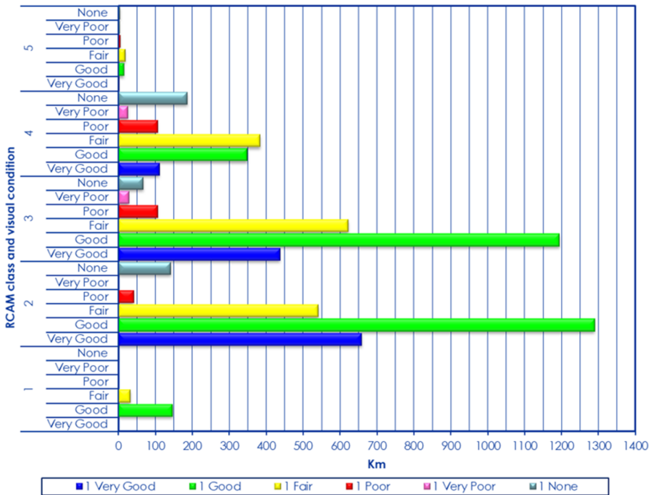
Figure 4-27: Condition of road markings according to RCAM class in June 2020
