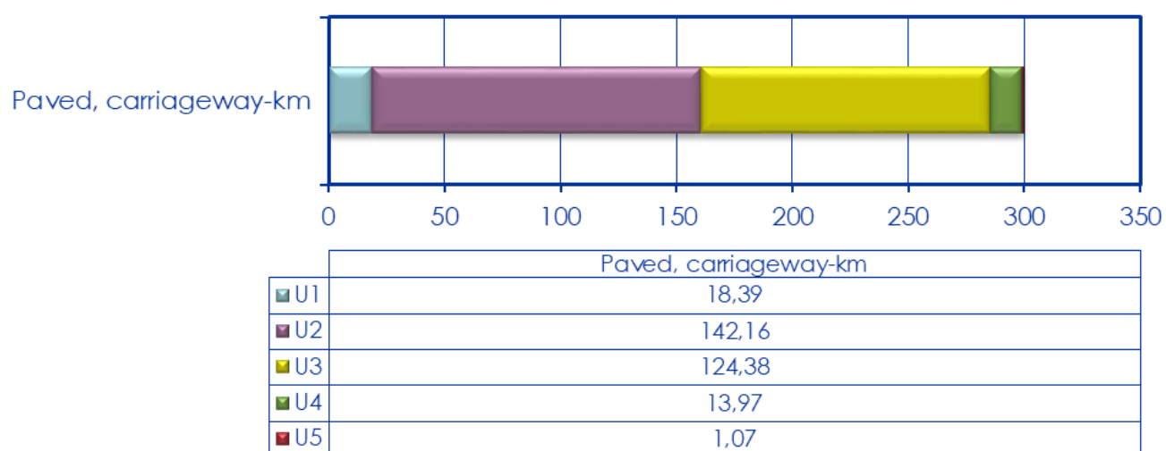
Figure 2-2: The urban WCG proclaimed municipal main road network classification according to TRH 26 (June 2020)
