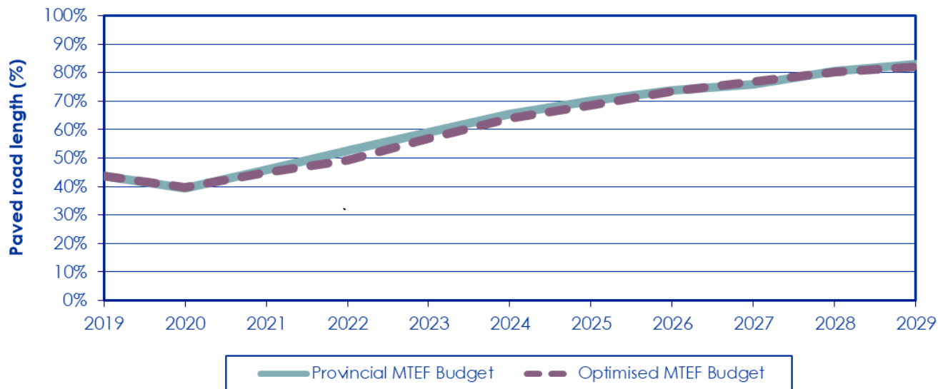
Figure 5-24: Percentage length of the paved road network not meeting the minimum intervention levels
