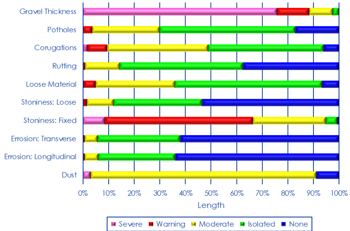
Figure 4-39: Condition distribution of the distresses on the unpaved road network as at December 2019
