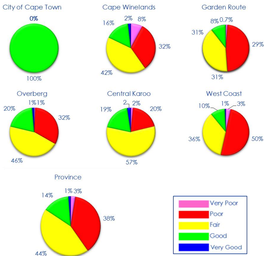
Figure 4-11: Condition distribution per kilometre by DM area for unpaved roads as at December 2019
