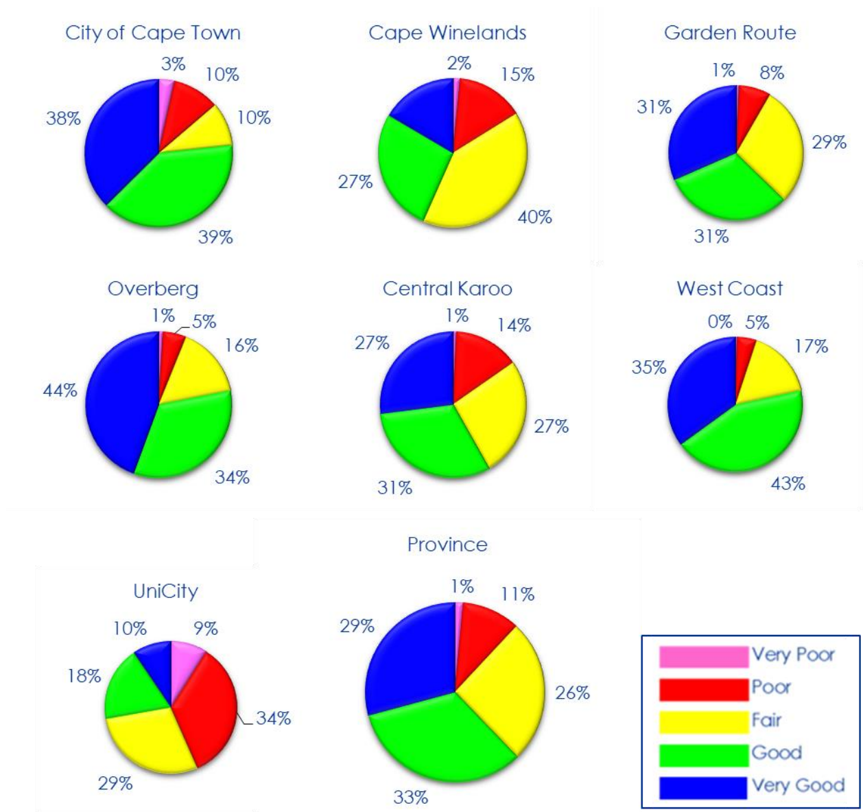
Figure 4-7: Condition distribution per kilometre by DM area for paved roads as at December 2019 including UniCity roads
