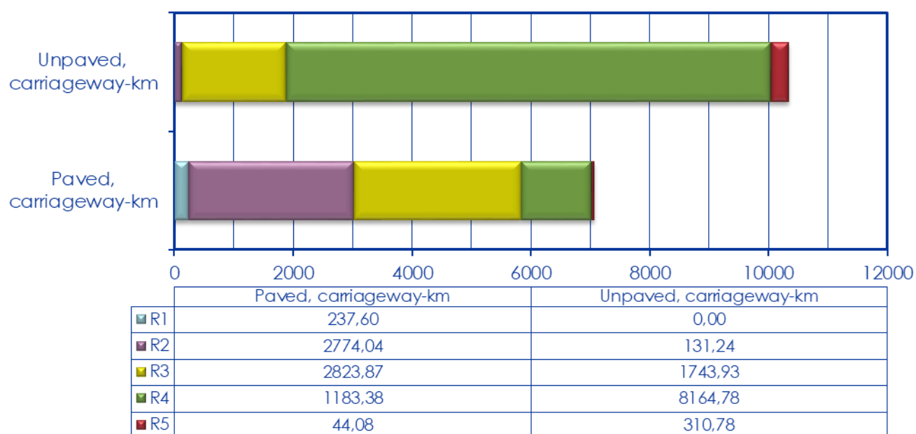
Figure 2-1: The WCG maintained rural road network classification according to TRH 26 (June 2020)
