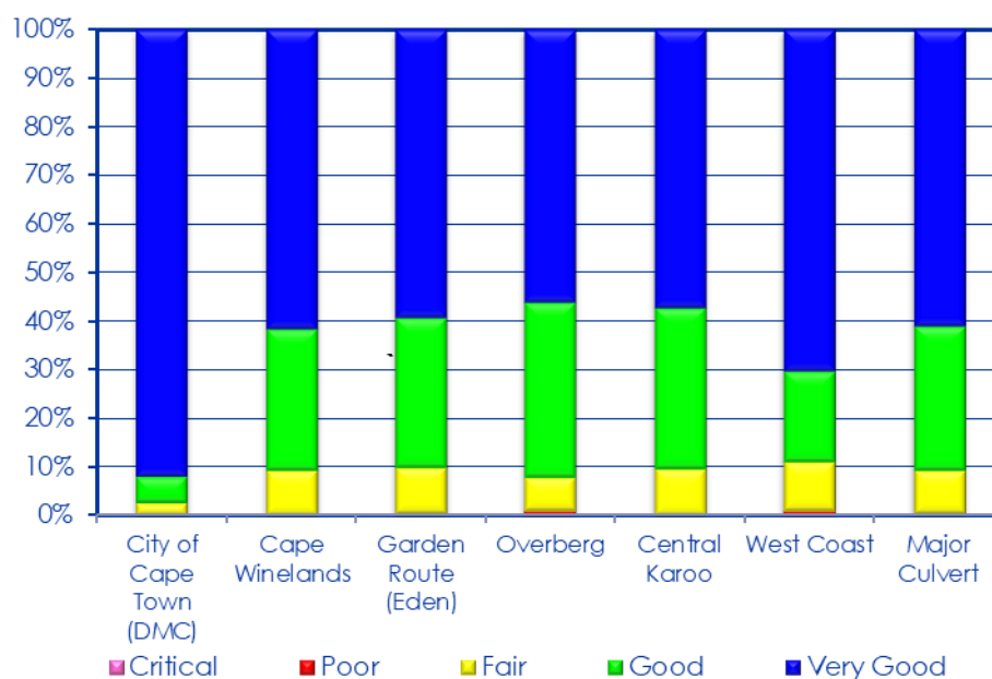
Figure 4-18: ACI for major culverts per DM (March 2020)
