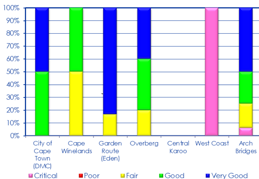
Figure 4-22: PCI for arch bridges per DM (March 2020)
