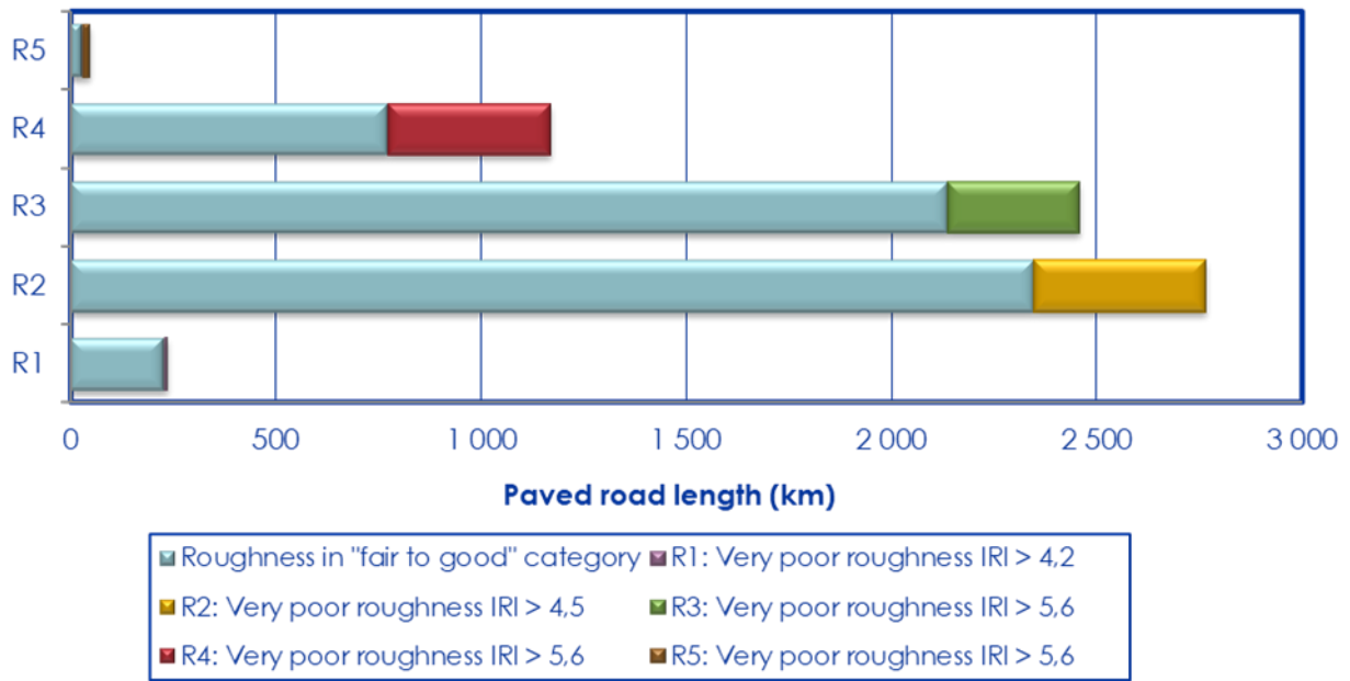
Figure 5-6: Proportion of paved roads that do not comply with minimum standards for roughness in 2016 based on the 2019 length
