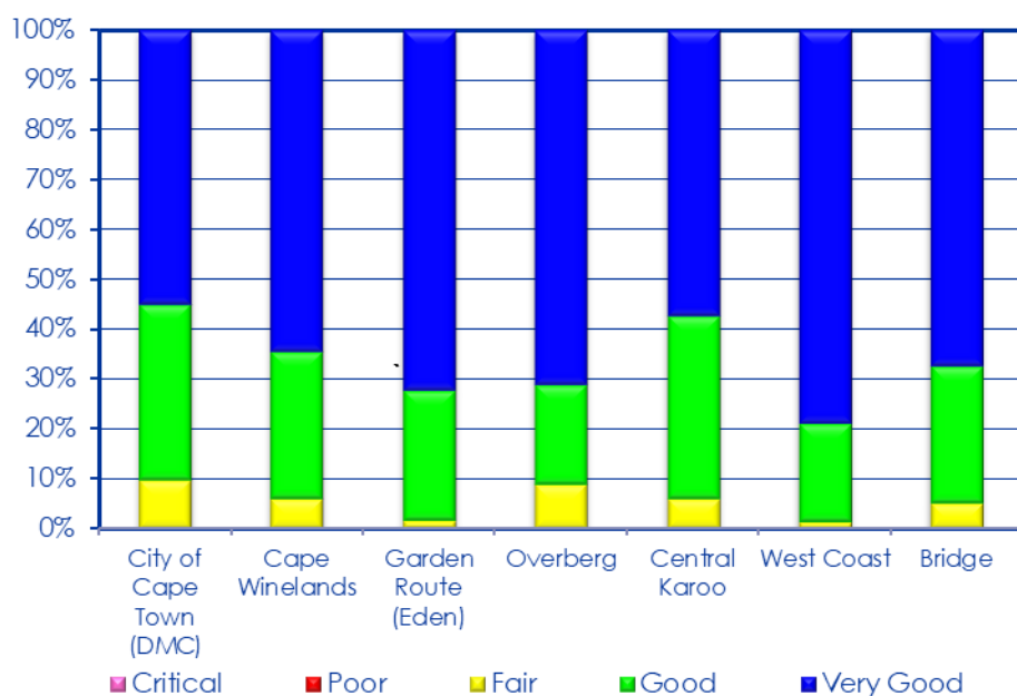
Figure 4-15: ACI for bridges per DM (March 2020)
