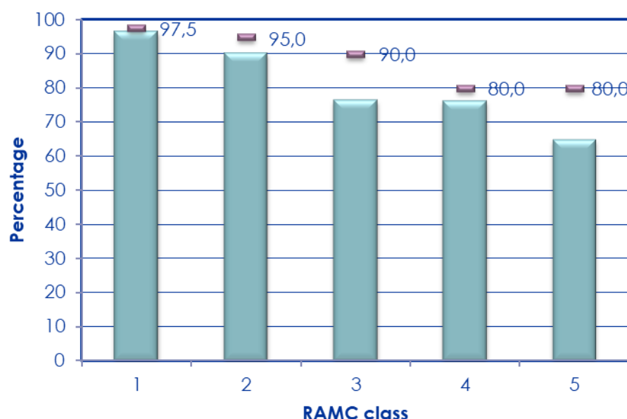
Figure 4-35: Smooth travel exposure per RCAM class compared with preliminary LOS targets for 2018
