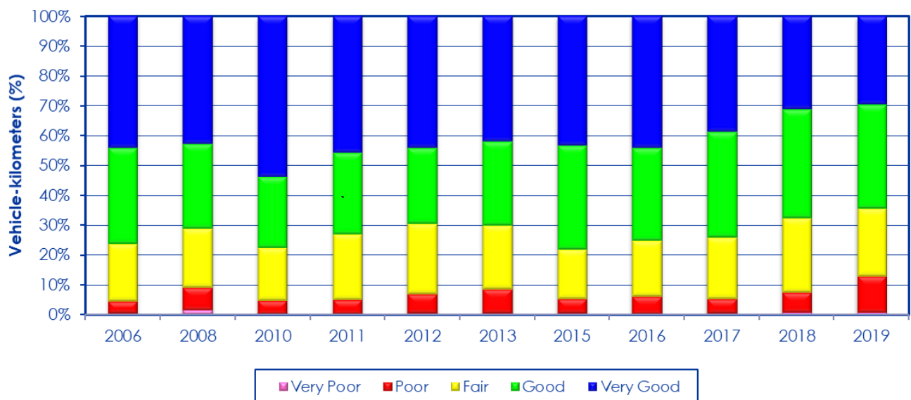
Figure 4-48: Distribution of the VCI of paved roads by annual vehicle-km travelled 2006 to 2019 (2019 including UniCity roads)
