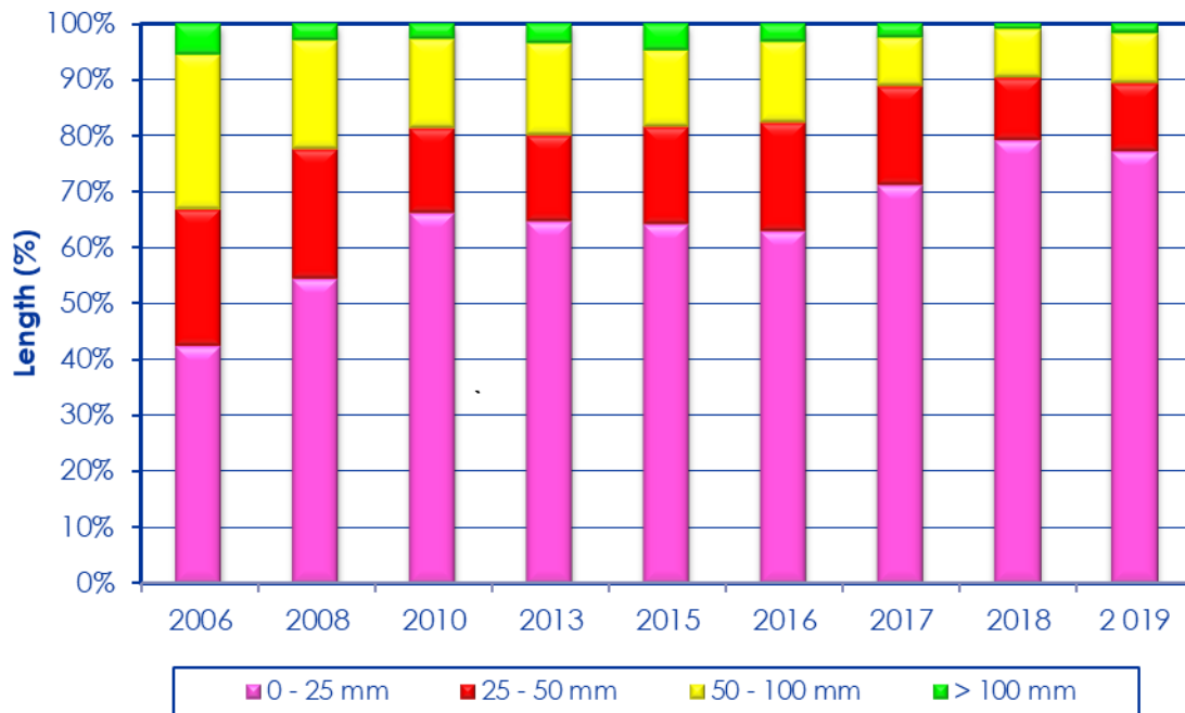
Figure 4-55: Gravel thickness distribution on unpaved roads 2006 to 2019
