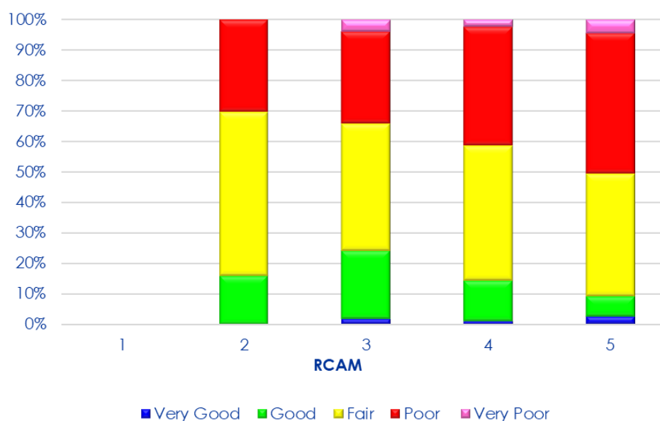
Figure 4-12: Condition distribution per kilometre by RCAM class for unpaved roads as at December 2019
