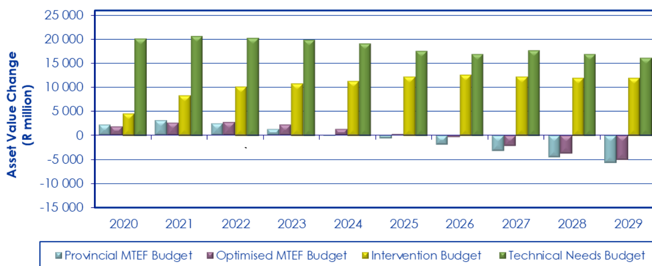
Figure 5-33: Change in asset value of the road network compared to 2019 value
