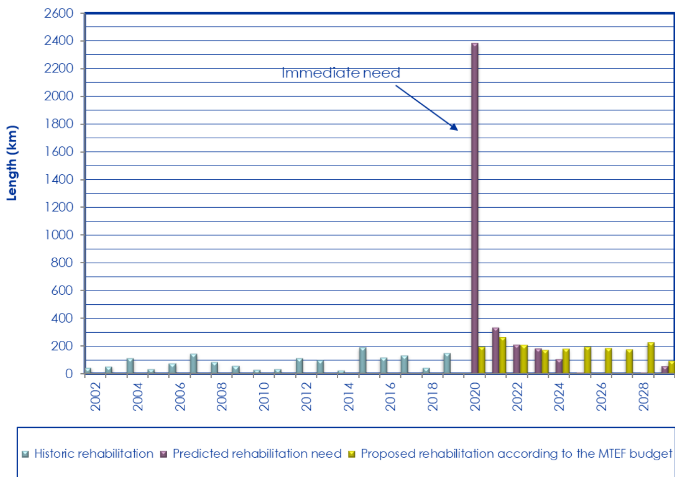
Figure 5-8: Historic rehabilitation of paved roads versus immediate rehabilitation need and proposed intervention of the MTEF budget for 2002 to 2030
