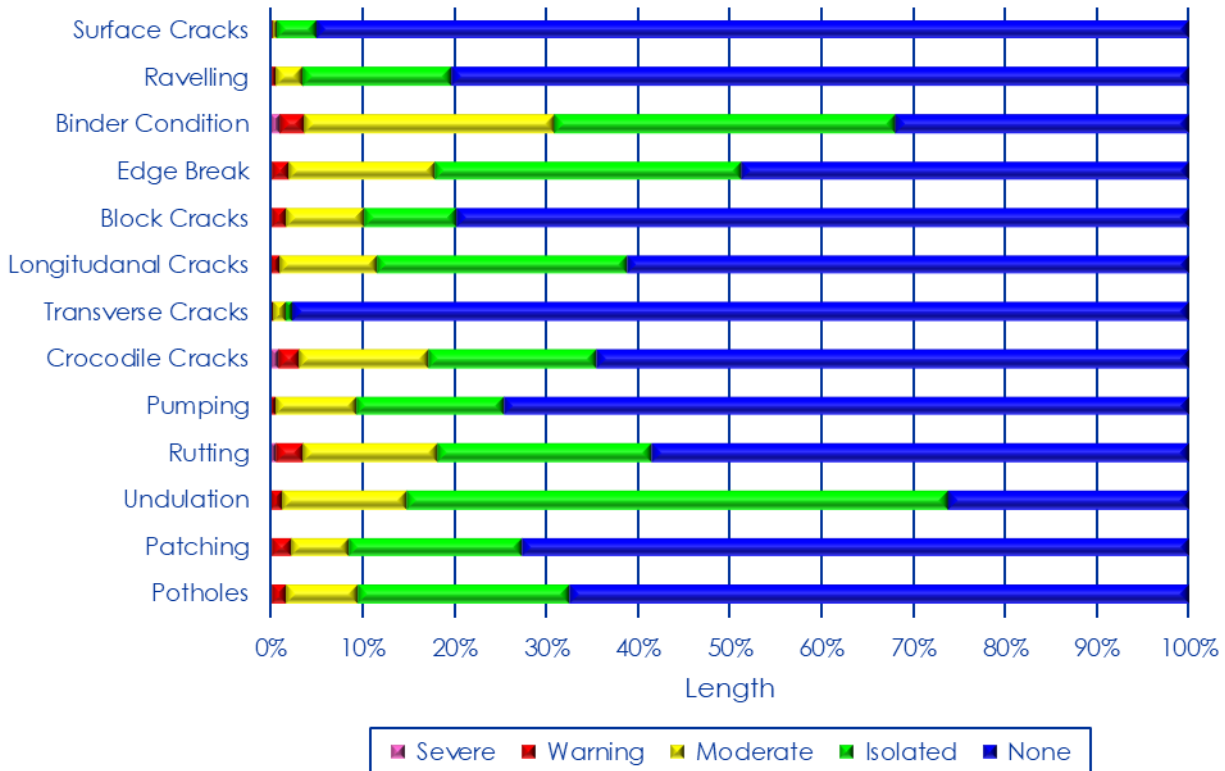
Figure 4-38: Condition distribution per distress for paved roads as at December 2019
