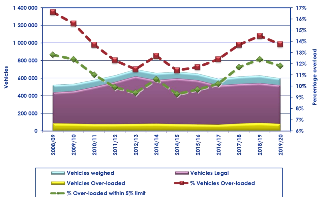
Figure 2-3: Historical trend of vehicles weighed
