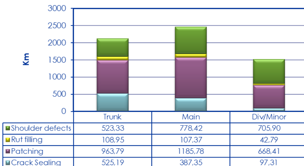
Figure 5-3: Maintenance demand in km of road according to road category 2019
