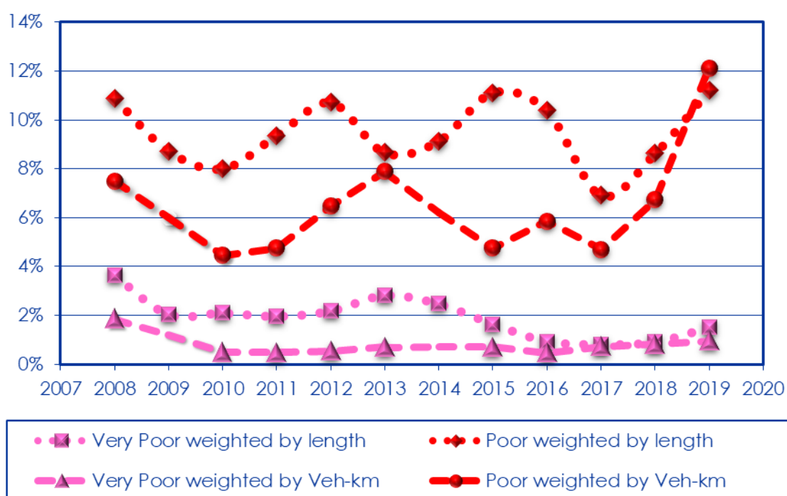
Figure 4-49: The percentage length of paved roads in a poor and very poor visual condition weighted by length and by vehicle-kilometres 2008 to 2019
