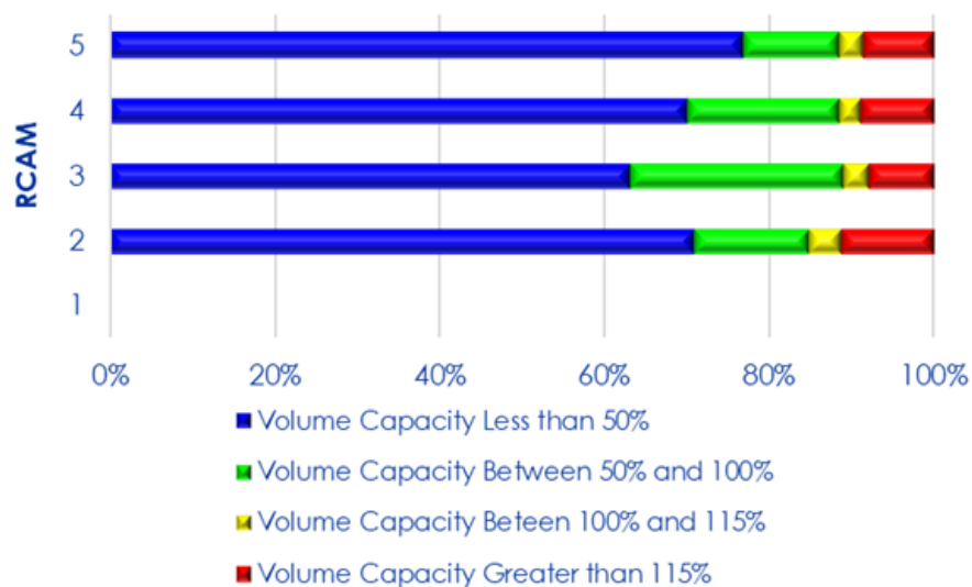
Figure 4-32: Volume capacity ratio for unpaved roads
