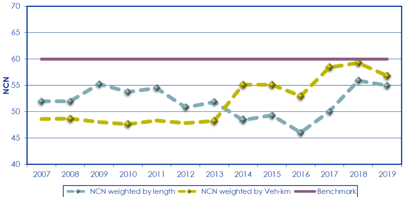
Figure 4-53: The historic trend in the overall network condition of maintained unpaved roads 2007 to 2019
