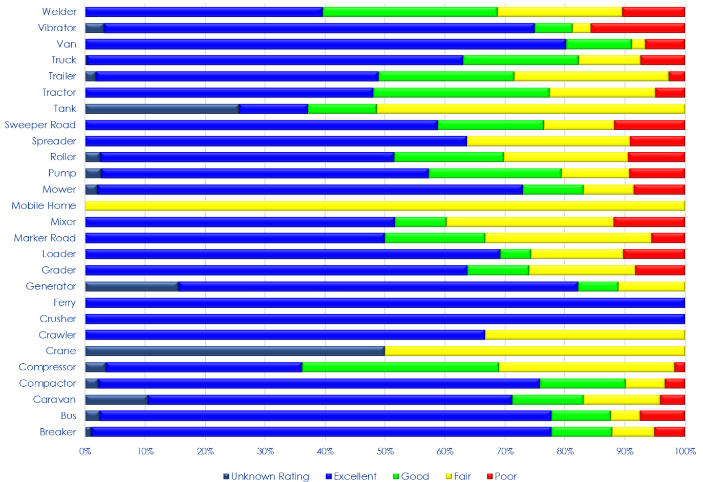
Figure 4-28: Condition distribution of the plant equipment
