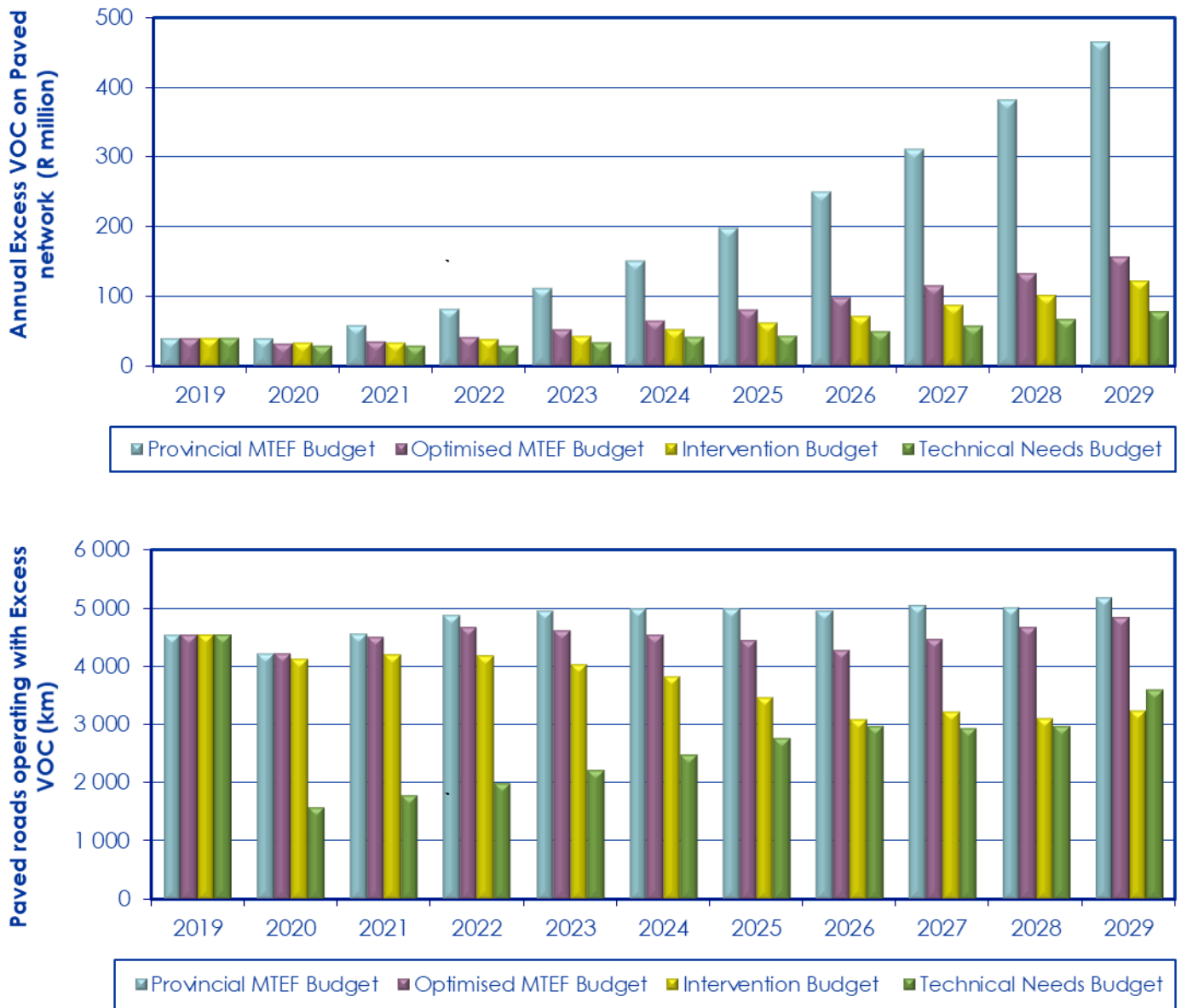
Figure 5-27: Total excess vehicle operating costs in terms of (a) annual cost and (b) km
