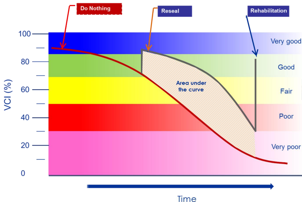
Figure 5-12: Illustration of Area-Under-the-Condition Curve
