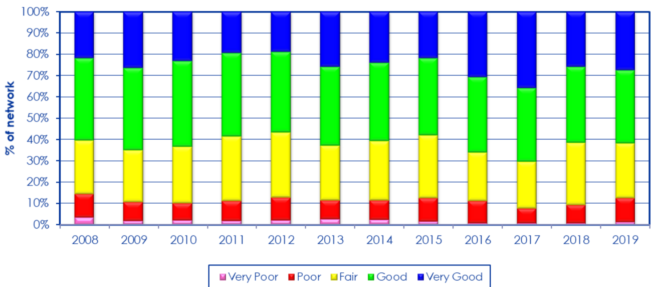
Figure 4-47: Change in the VCI by road length of the paved road network 2008 to 2019 (2019 including UniCity roads)
