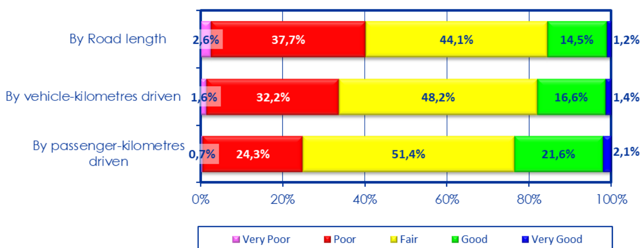
Figure 4-10: Unpaved roads condition distribution by length versus vehicle and passenger-kilometres in Dec. 2019
