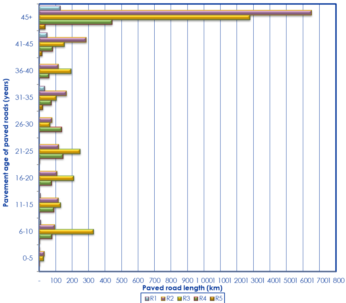
Figure 4-44: Distribution of pavement ages for paved roads 2019
