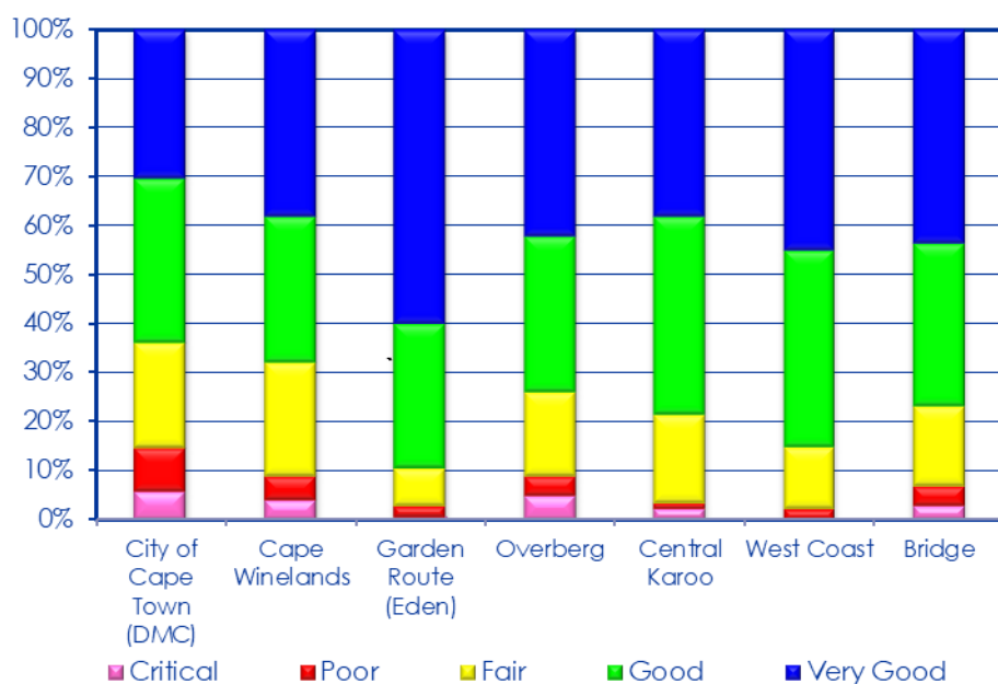
Figure 4-21: PCI for bridges per DM (March 2020)
