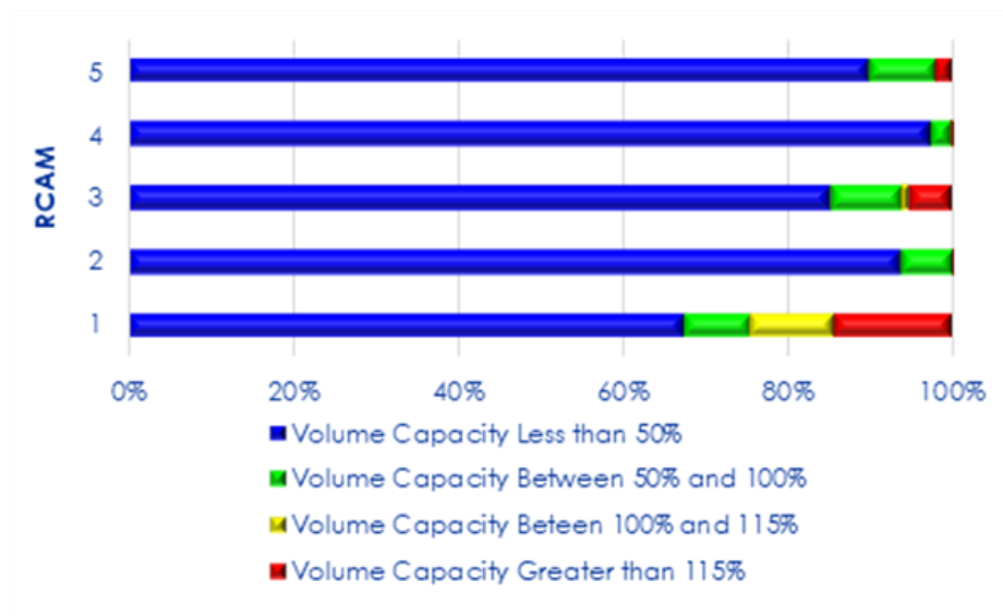
Figure 4-31: Volume capacity ratio for paved roads
