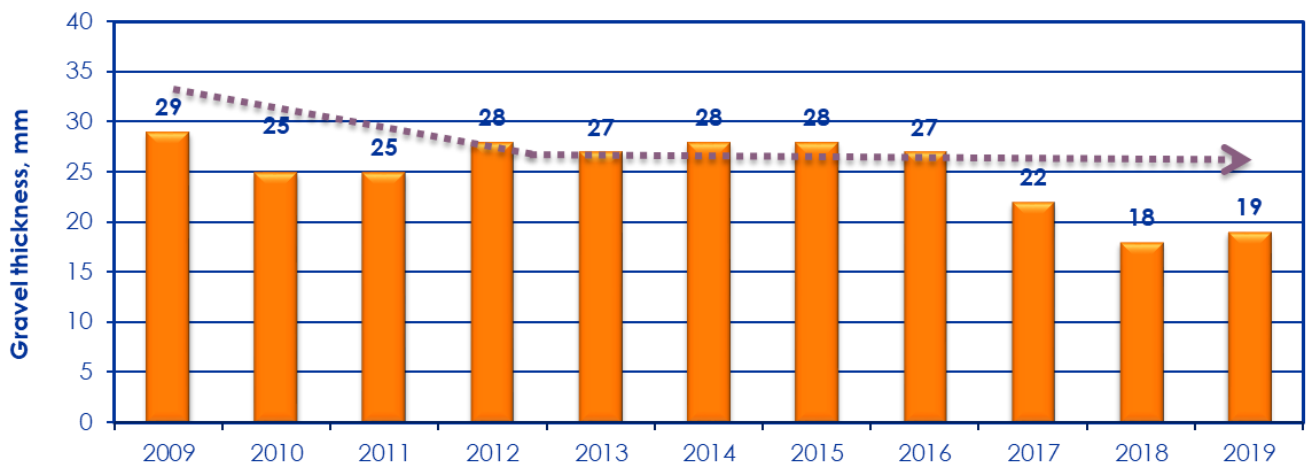
Figure 4-54: The historic trend in gravel thickness on the maintained unpaved road network from 2009 to 2019
