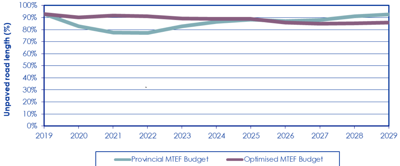
Figure 5-29: Length of the unpaved road network not meeting the minimum intervention levels
