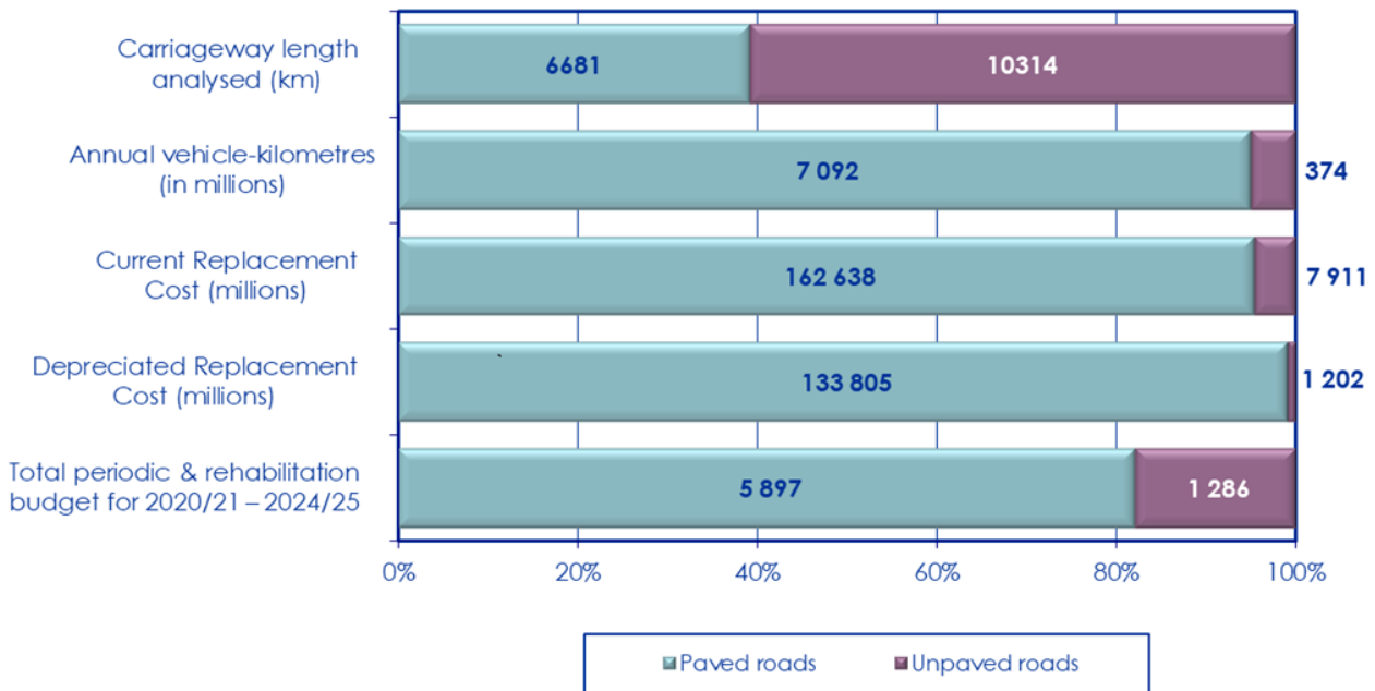
Figure 5-38: Comparison of paved and unpaved roads
