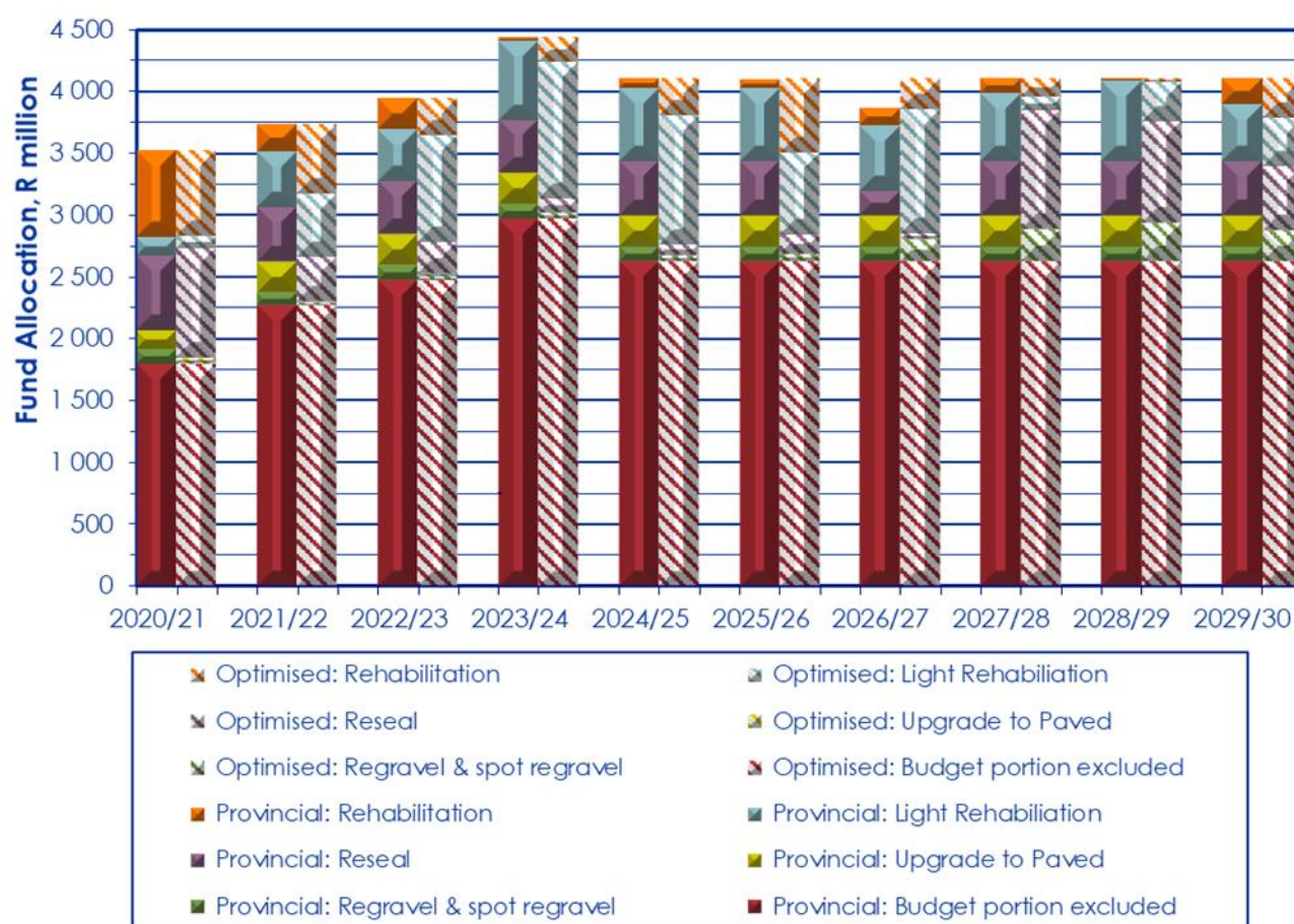
Figure 5-19: Provincial and optimised allocations of the MTEF funds over the next 10 years
