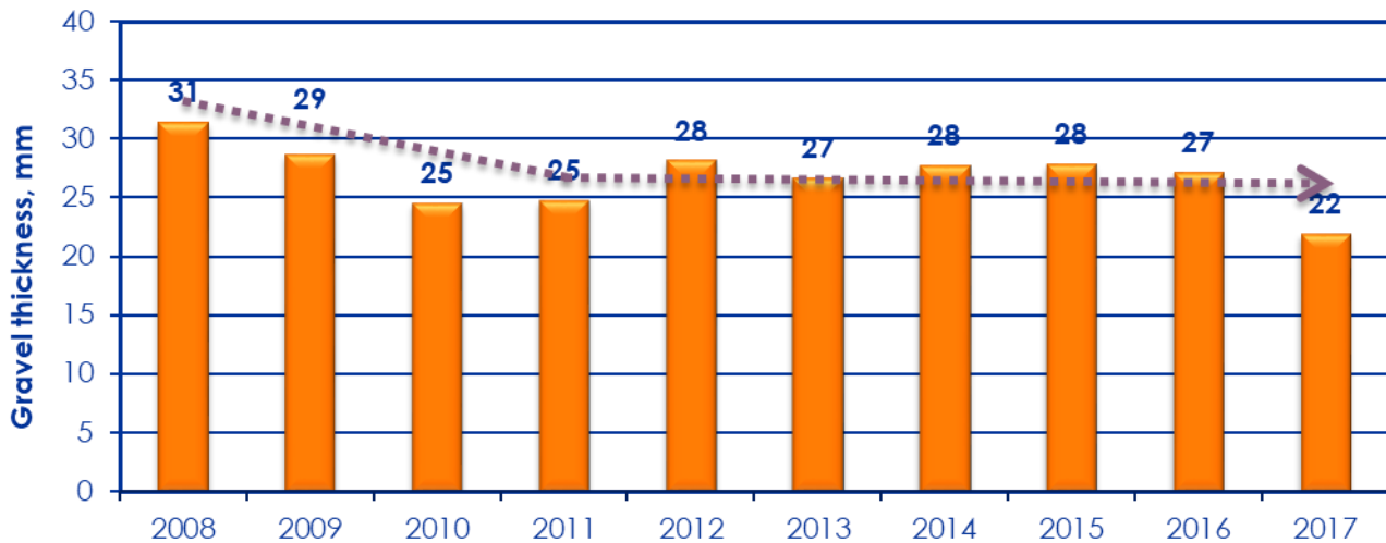
Figure 4-28: The historic trend in gravel thickness on the maintained unpaved road network from 2008 to 2017
