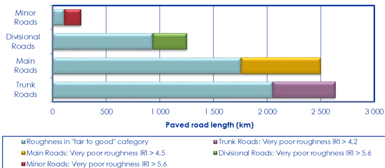
Figure 5-13: Proportion of paved roads that do not comply with minimum standards for roughness in 2016 based on the 2018 length
