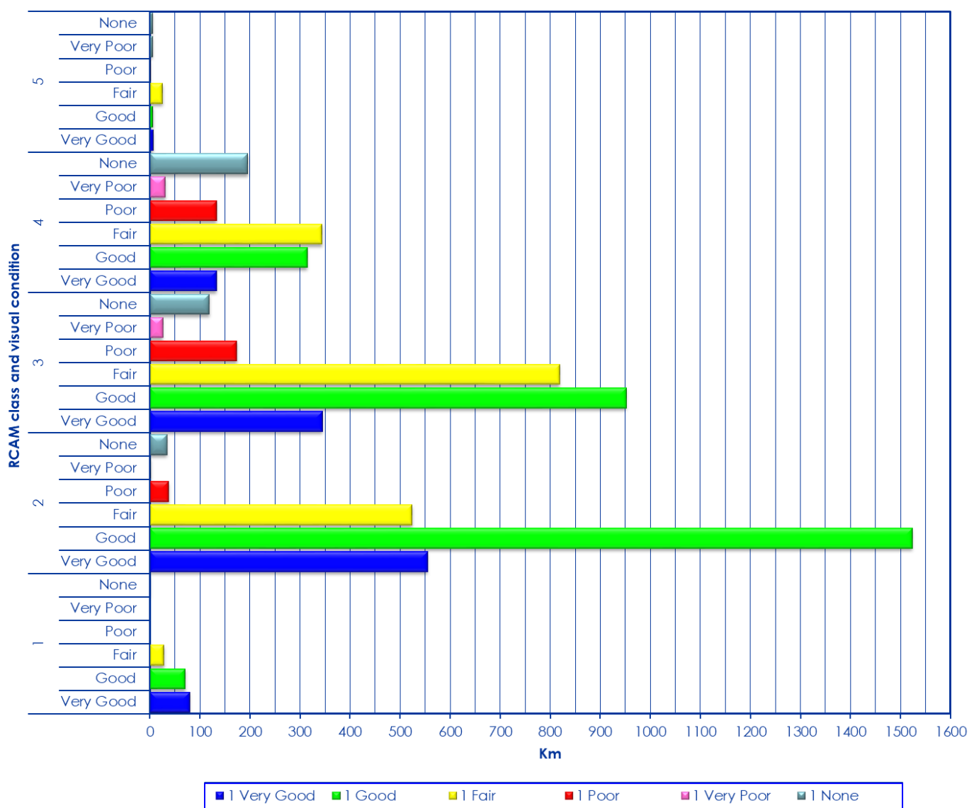
Figure 4-15: Condition of road markings according to RCAM class in 2017
