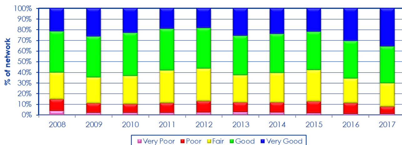
Figure 4-21: Change in the VCI by road length of the paved road network 2008 to 2017
