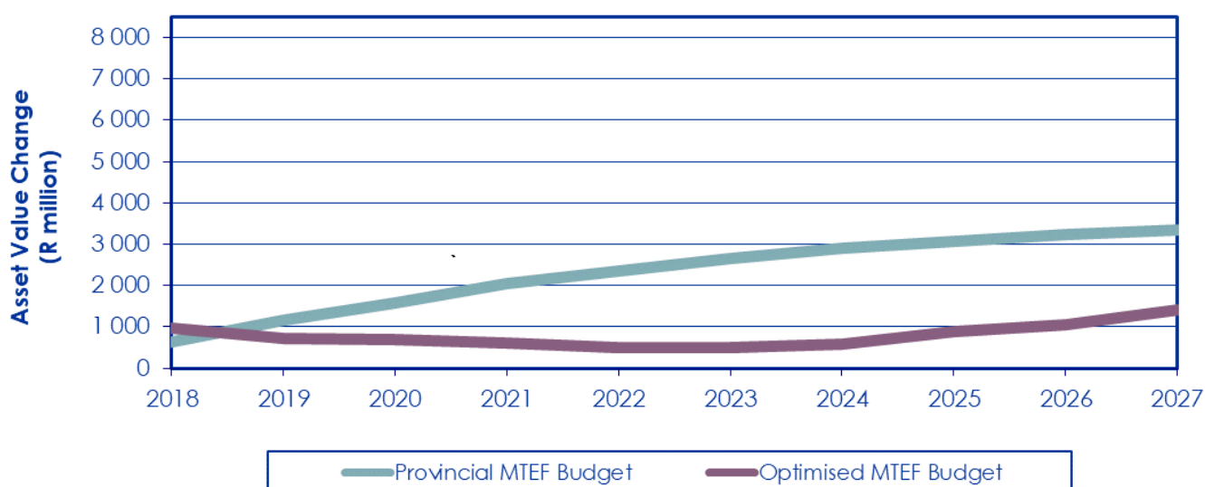
Figure 5-42: Change in asset value of unpaved roads
