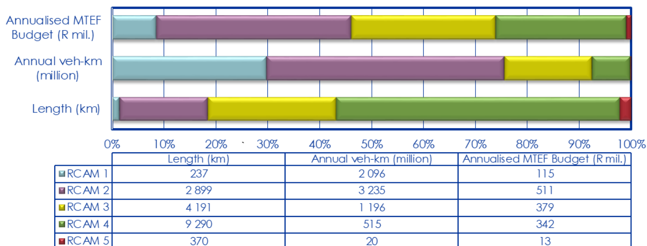
Figure 5-29: Road network according to RCAM classification versus the Optimised MTEF Budget allocation
