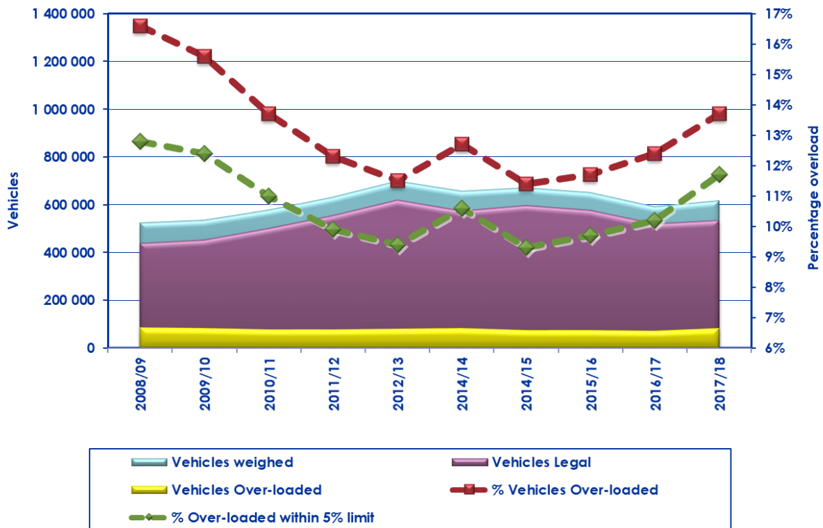
Figure 2-3: Historical trend of vehicles weighed
