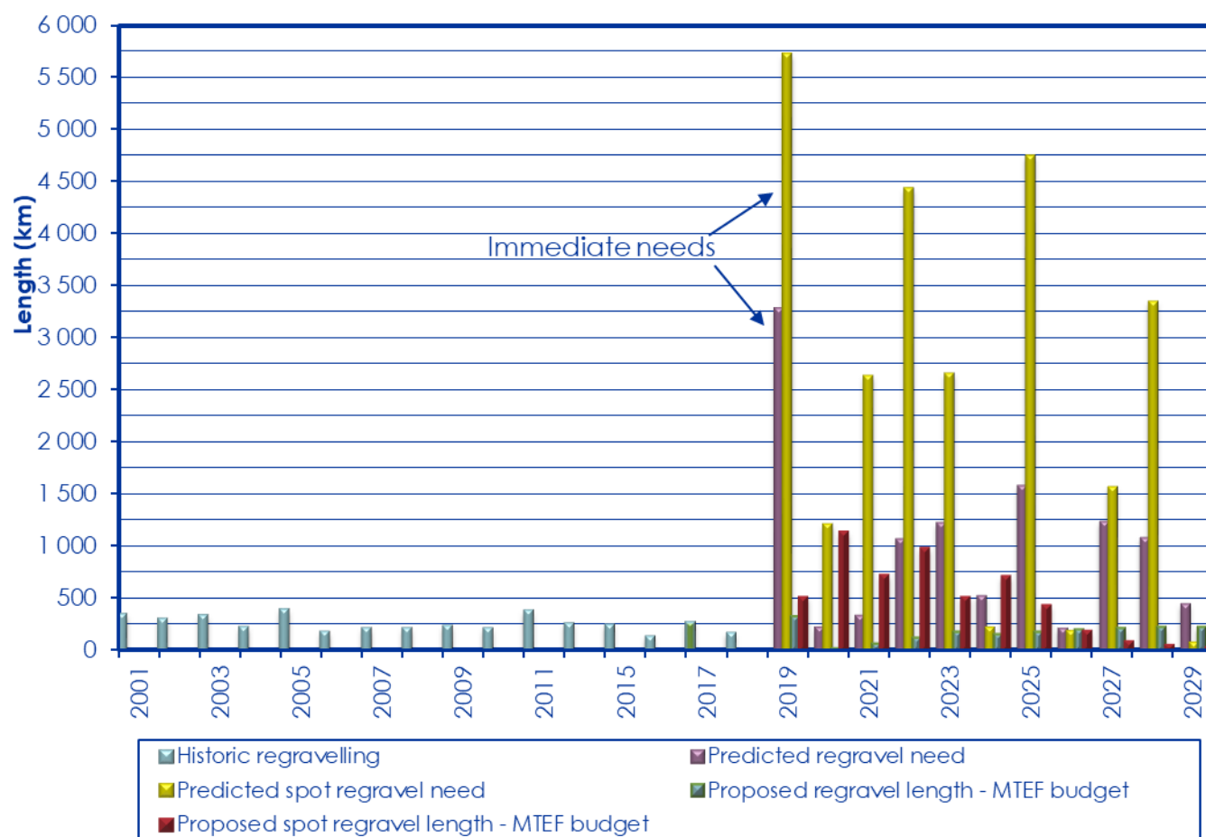
Figure 5-16: Historic regravelling of maintained unpaved roads versus immediate need and proposed intervention of the MTEF budget for 2001 to 2029
