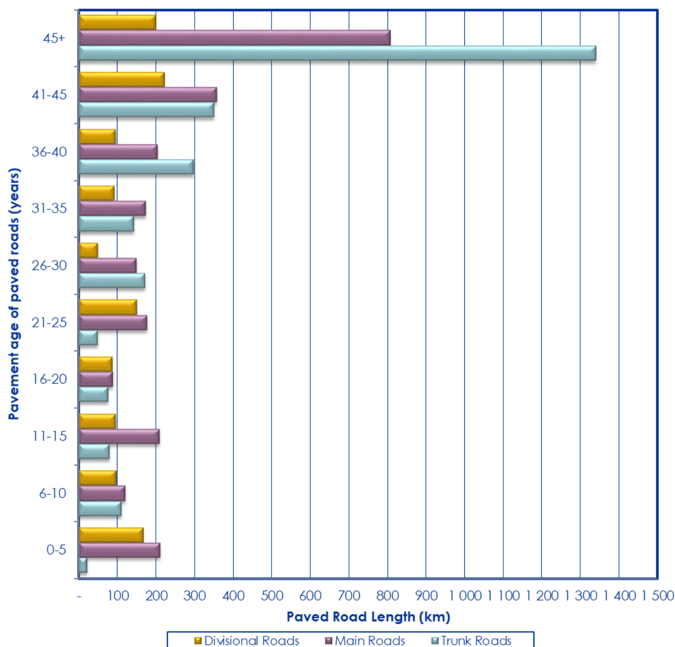
Figure 5-6: Distribution of pavement ages for paved roads 2017
