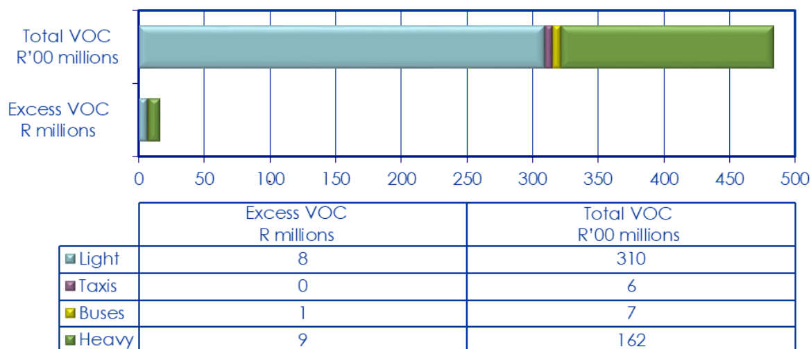
Figure 4-18: Total and excess vehicle operating costs on paved roads for 2017
