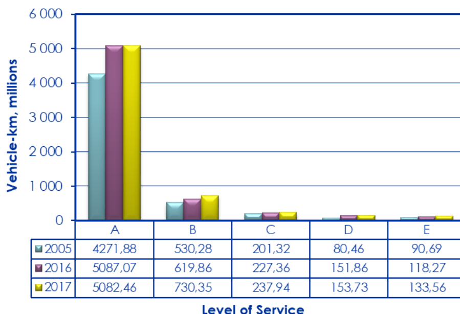
Figure 4-8: Vehicle-km travelled annually for each level of service category in 2005, 2016 and 2017
