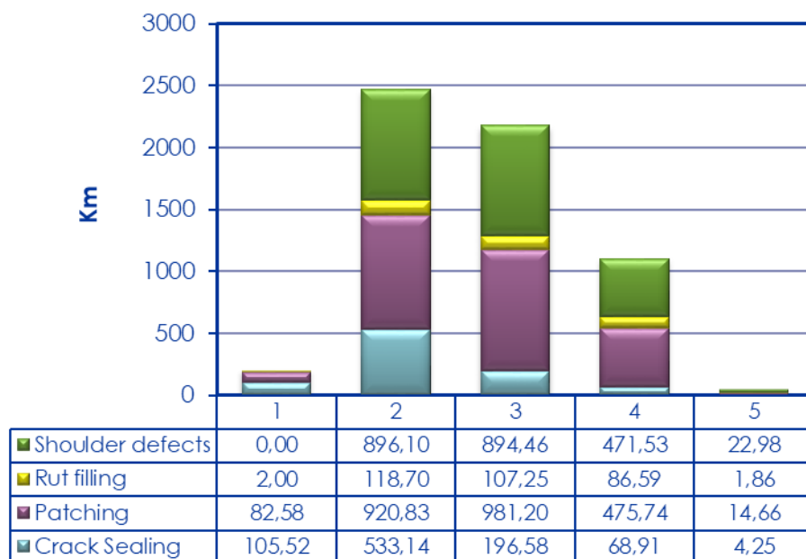
Figure 5-11: Maintenance demand in km of road according to road category 2017
