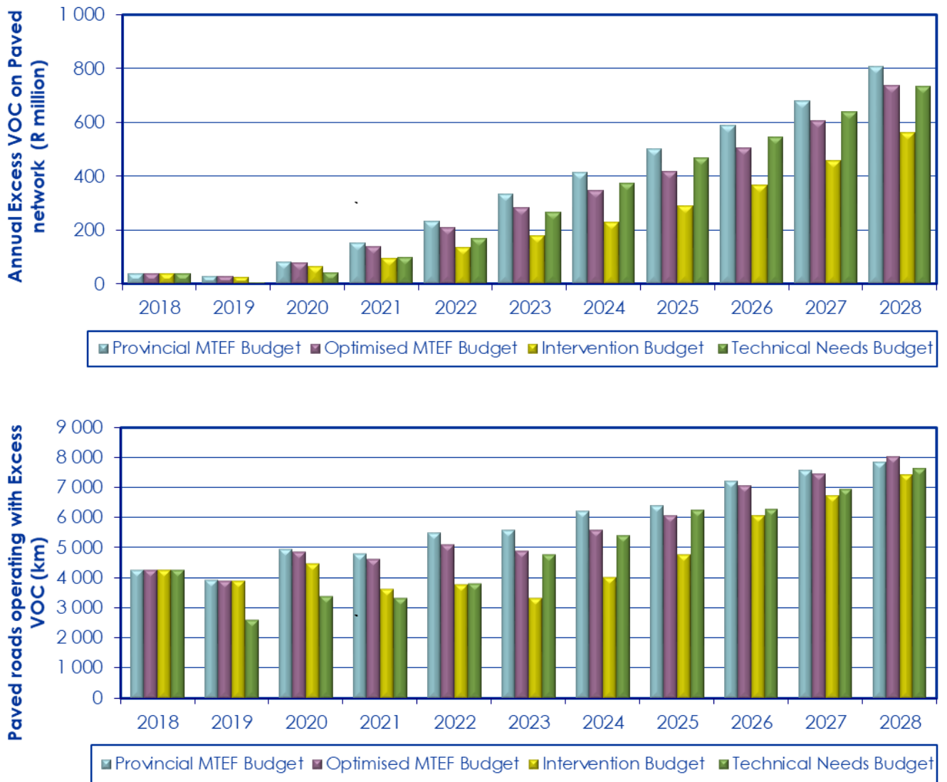
Figure 5-34: Total excess vehicle operating costs in terms of (a) annual cost and (b) km
