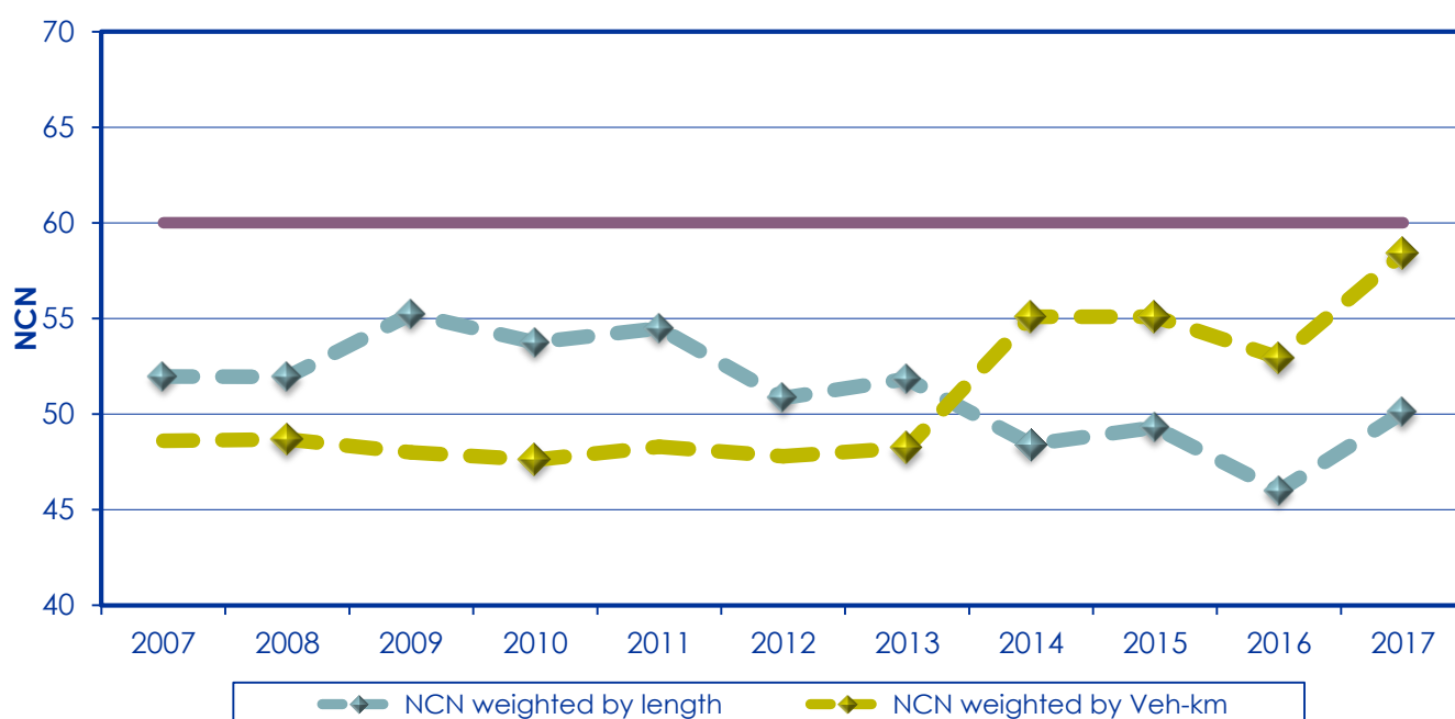
Figure 4-27: The historic trend in the overall network condition of maintained unpaved roads 2007 to 2017
