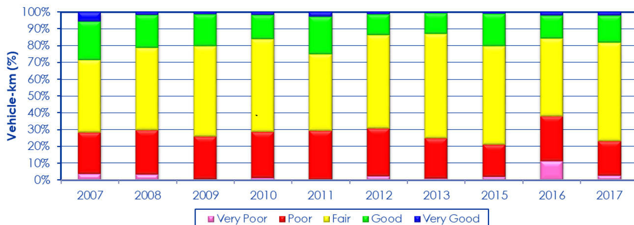
Figure 4-26: Distribution of the VCI of maintained unpaved roads by annual vehicle-km travelled 2007 to 2017
