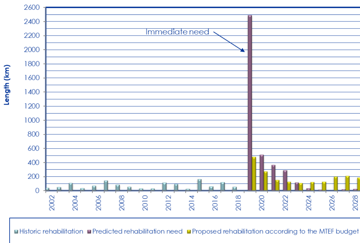
Figure 5-15: Historic rehabilitation of paved roads versus immediate rehabilitation need and proposed intervention of the MTEF budget for 2002 to 2028
