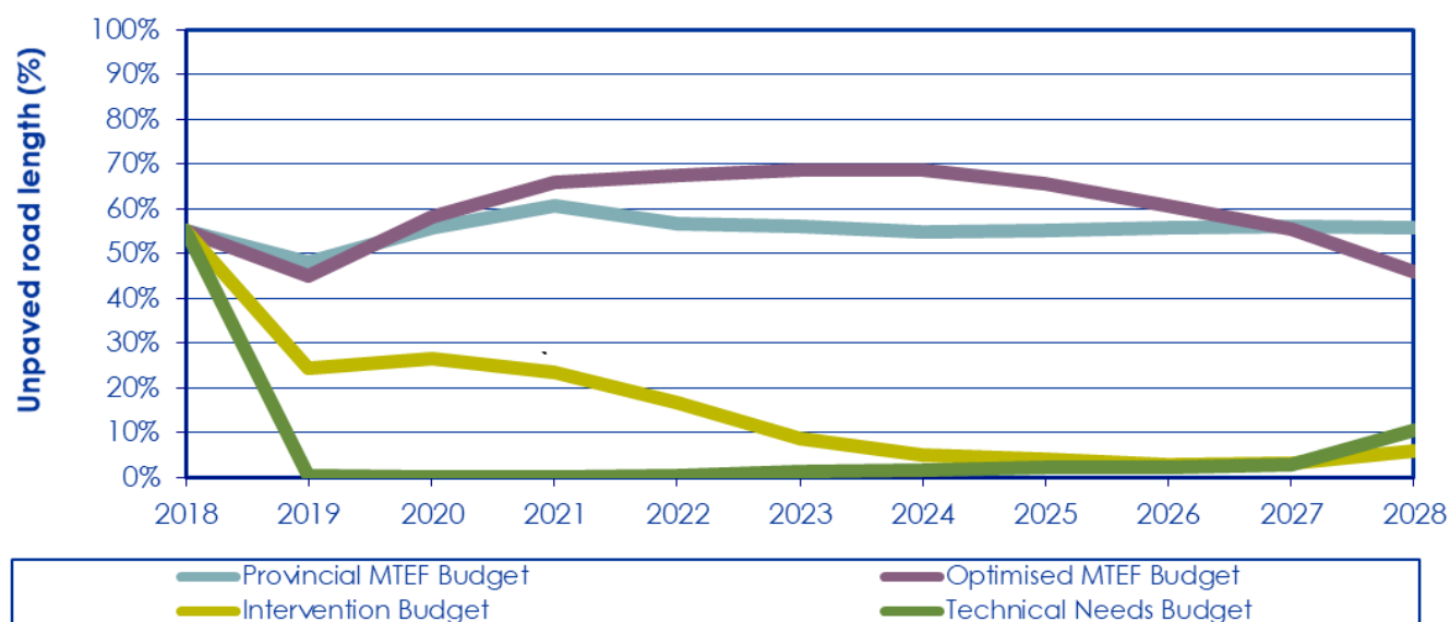
Figure 5-37: Proportion of unpaved roads without gravel, excluding earth roads
