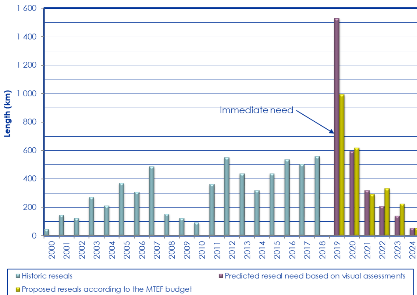
Figure 5-8: Historic resealing of paved roads versus the predicted need and proposed MTEF budget resealing programme from 2000 to 2024
