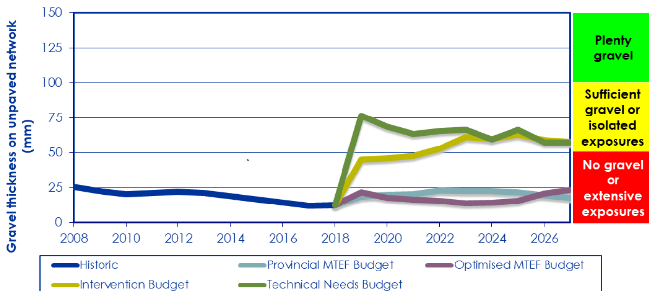
Figure 5-35: Average gravel thickness of maintained unpaved roads
