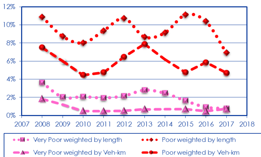
Figure 4-23: The percentage length of paved roads in a poor and very poor visual condition weighted by length and by vehicle-kilometres 2008 to 2017
