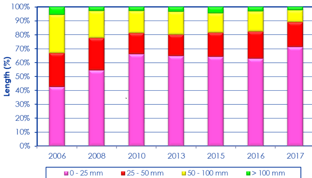
Figure 4-29: Gravel thickness distribution on unpaved roads 2006 to 2017
