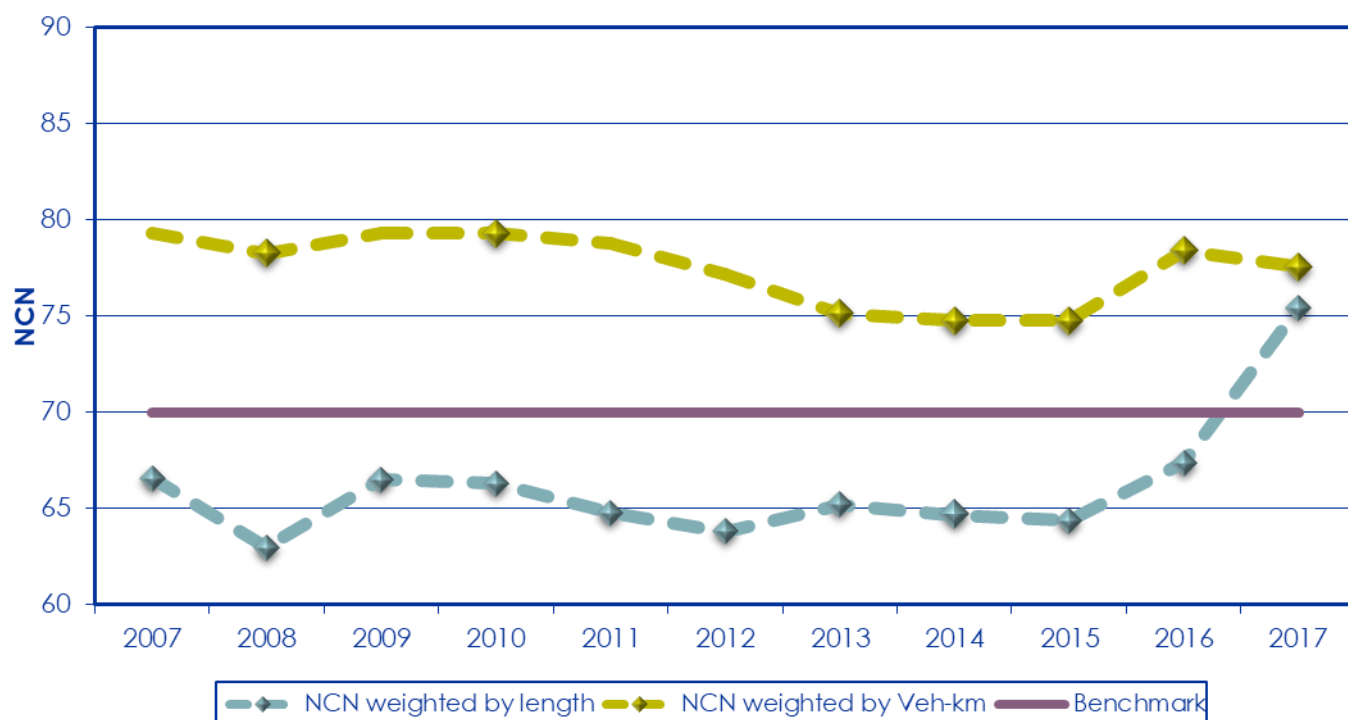
Figure 4-24: The historic trend in the overall network condition of the paved road network 2007 to 2017
