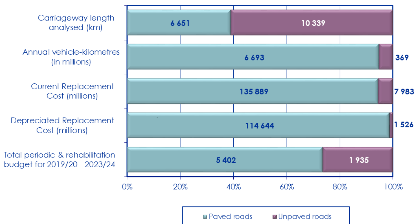
Figure 5-45: Comparison of paved and unpaved roads
