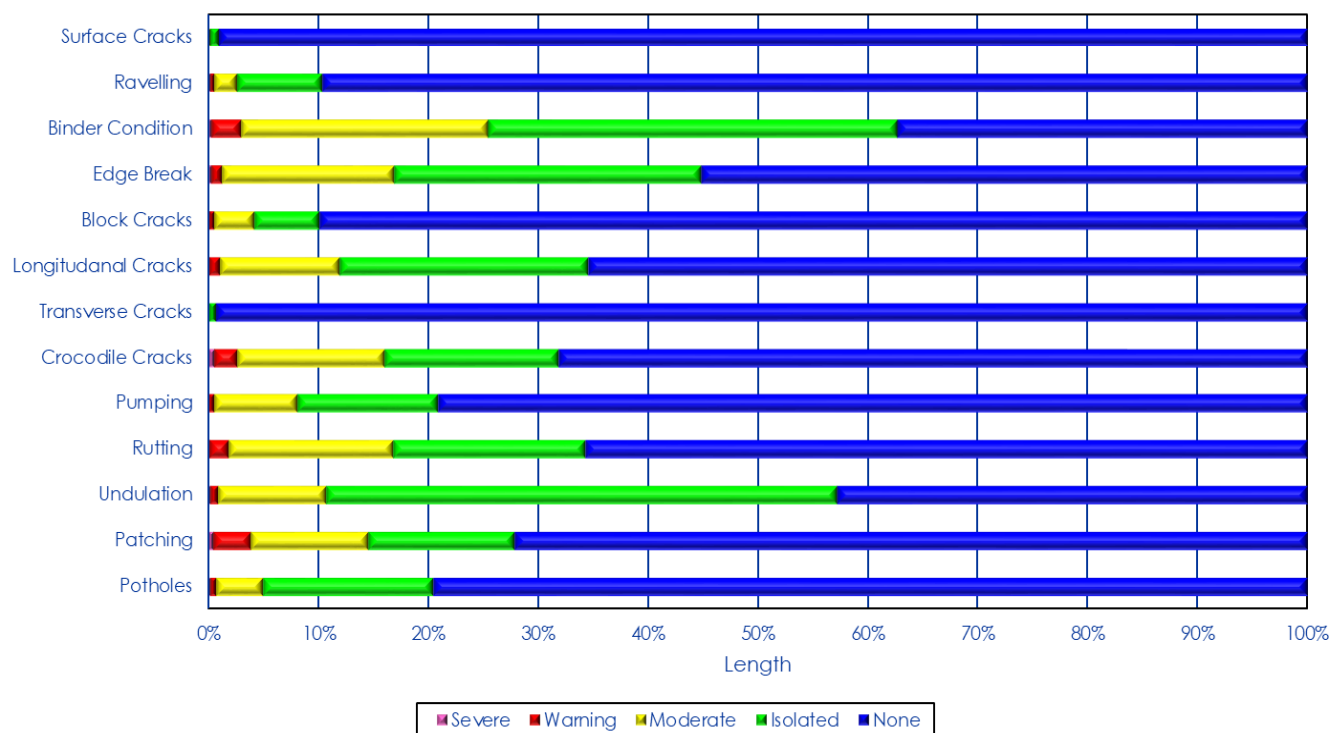
Figure 4-16: Condition distribution per distress for paved roads as at June 2017
