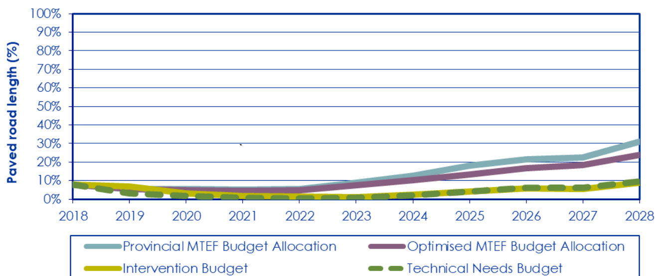
Figure 5-32: Percentage length of paved roads in poor and very poor condition
