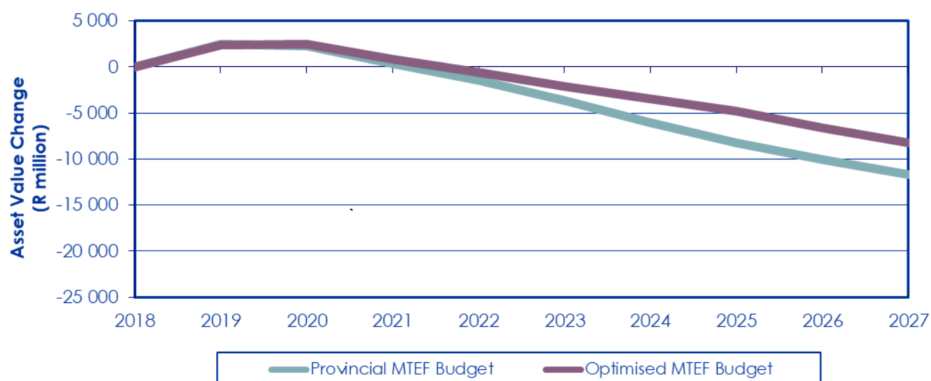
Figure 5-41: Change in asset value of paved roads
