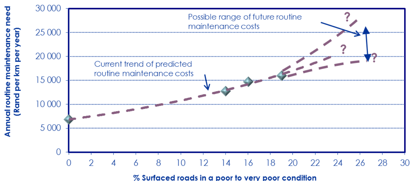
Figure 5-46: Routine maintenance cost versus condition of the paved road network
