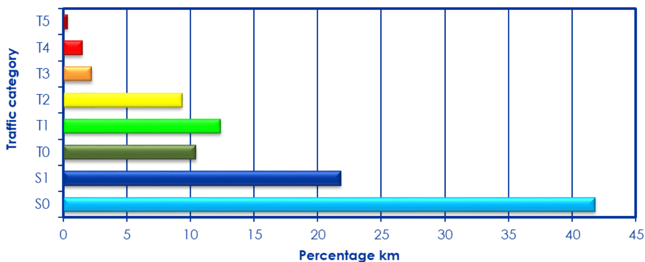
Figure 5-2: Traffic categories and their percentage of km of the network for 2017
