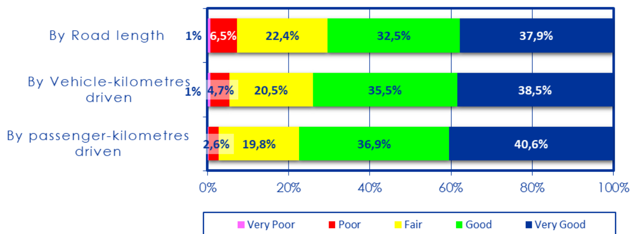
Figure 4-3: Paved roads condition distribution as at 30 June 2017
