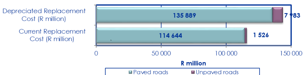
Figure 4-20: Current replacement and depreciated replacement costs of the road network in 2018
