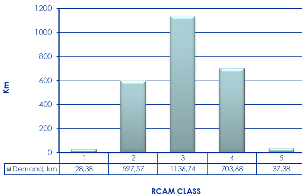
Figure 5-12: Demand for line marking where condition is fair or worse in 2017
