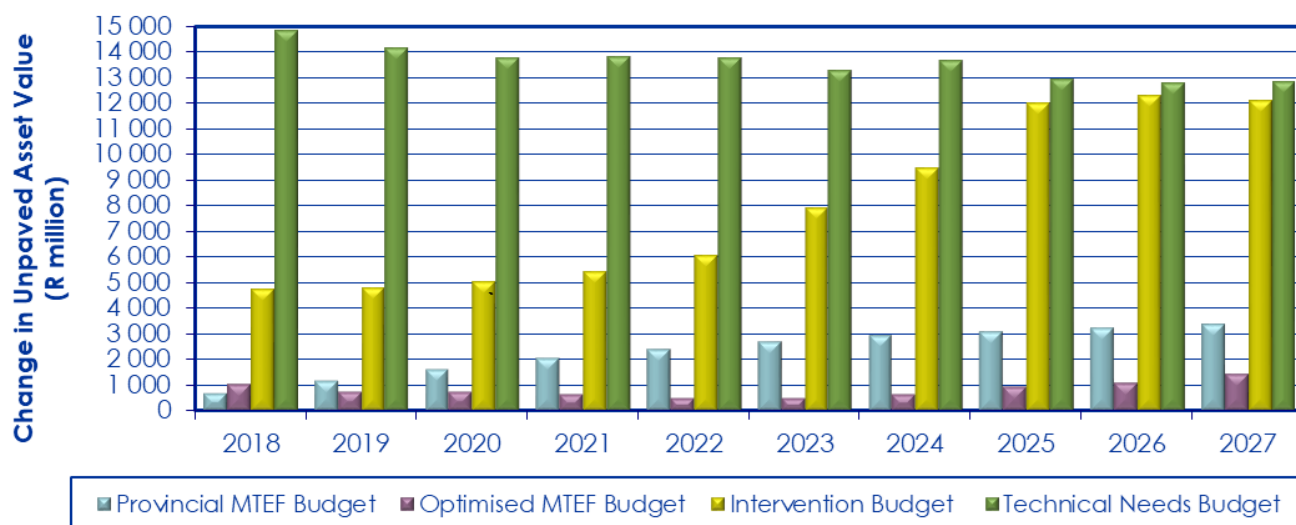
Figure 5-39: Change in asset value of maintained unpaved roads compared to 2017 values
