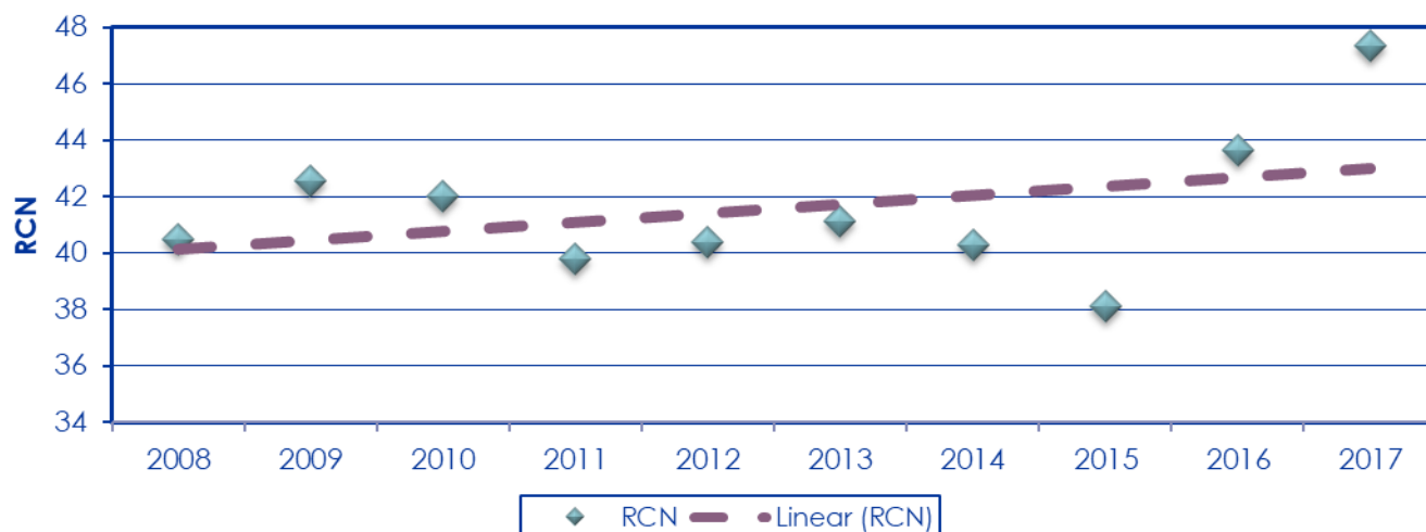
Figure 4-31: Historic trend of reseal condition number 2008 to 2017
