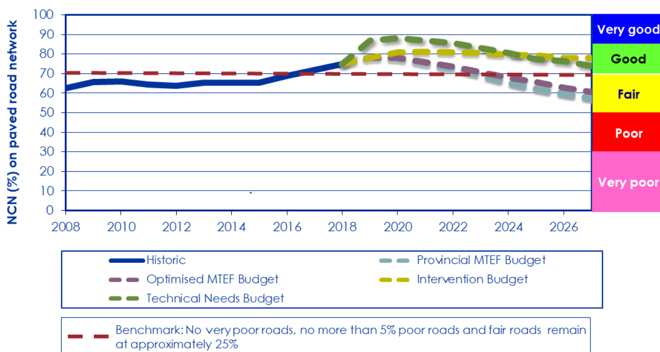
Figure 5-30: Average network condition of paved roads
