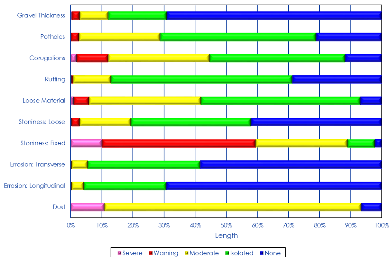
Figure 4-17: Condition distribution of the distresses on the unpaved road network as at June 2017
