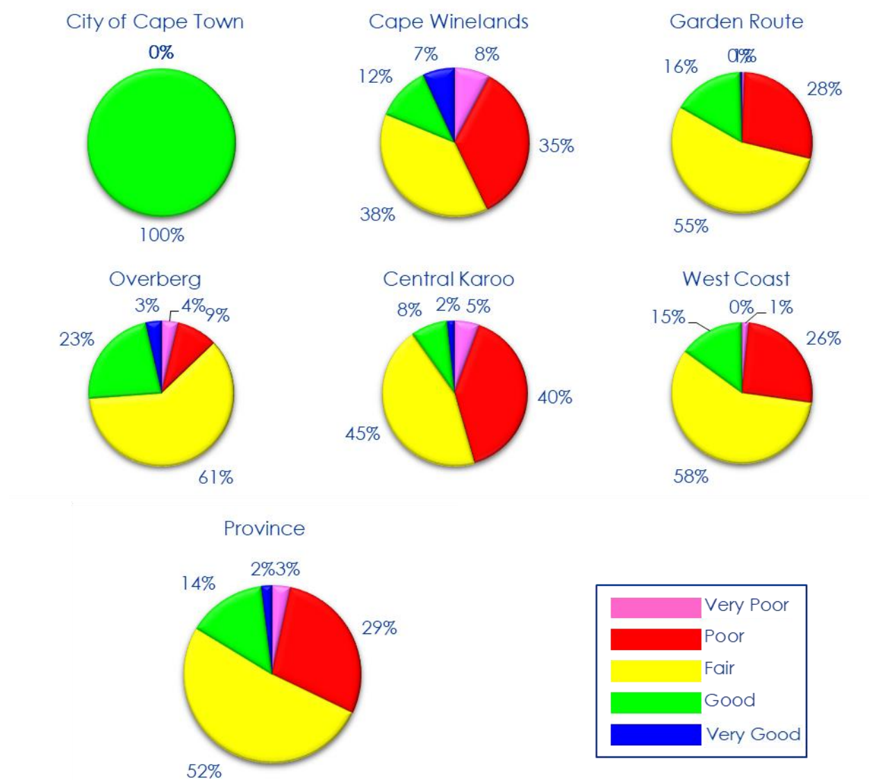
Figure 4-7: Condition distribution per kilometre by DM area for unpaved roads as at June 2017
