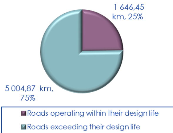
Figure 5-5: Pavement ages versus design life in 2017
