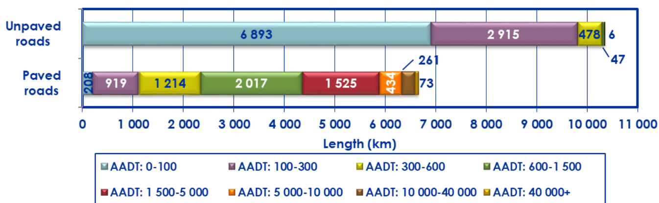
Figure 5-3: Traffic distribution on paved and unpaved roads 2017
