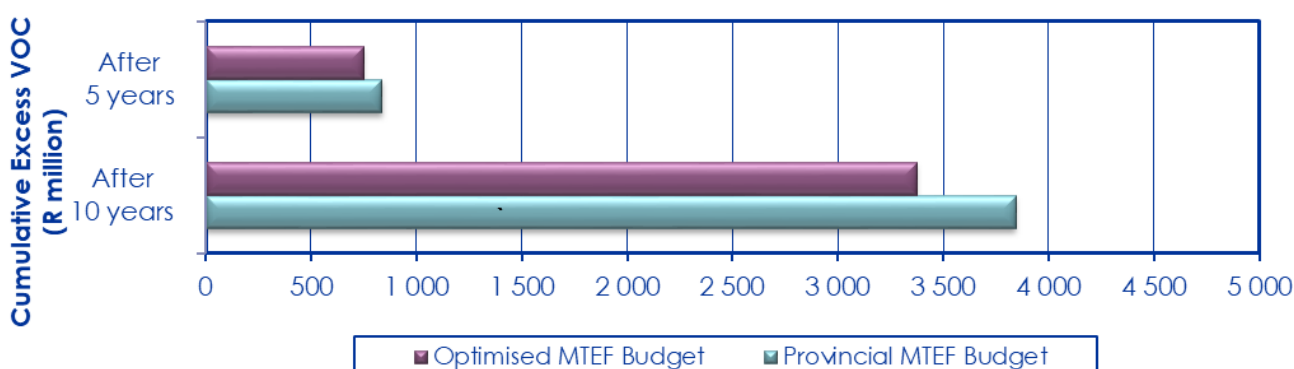
Figure 5-43: Total excess vehicle operating costs for the current funding levels on paved roads
