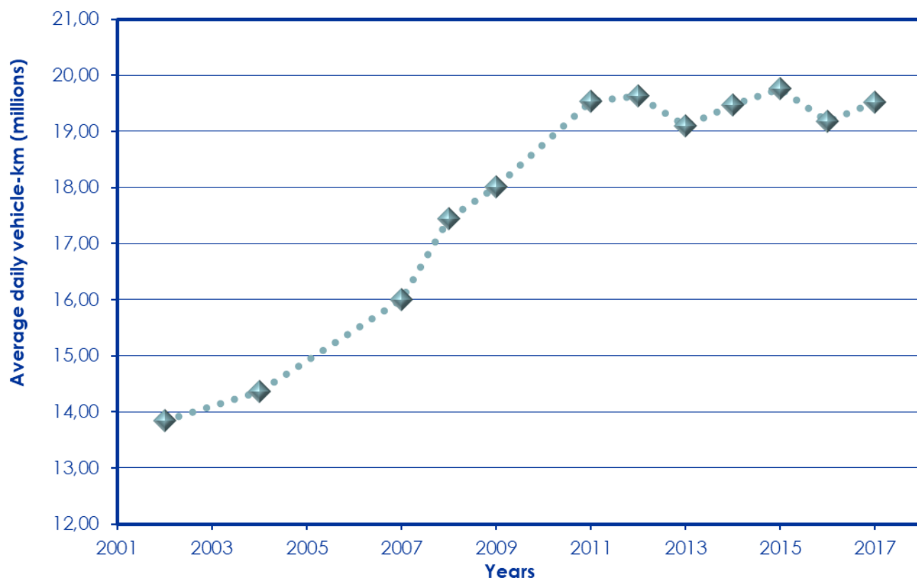
Figure 5-1: Growth in average daily vehicle-km on the WCG network 2002 to 2017
