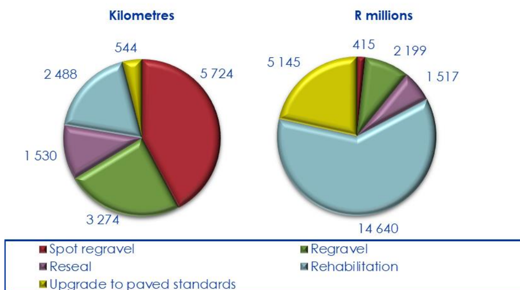
Figure 5-44: Immediate need according to the Technical Needs Budget
