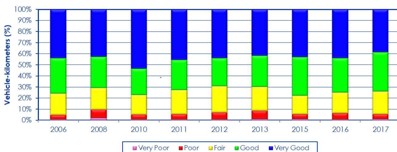
Figure 4-22: Distribution of the VCI of paved roads by annual vehicle-km travelled 2006-2017
