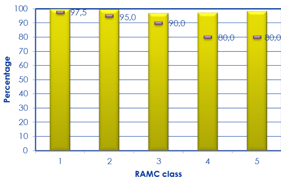
Figure 4-11: Low rut exposure per RCAM class compared with preliminary LOS targets for 2015
