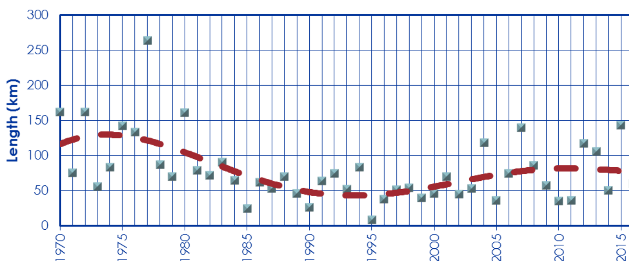
Figure 5-7: Rate of rehabilitation for paved roads 1970 to 2016
