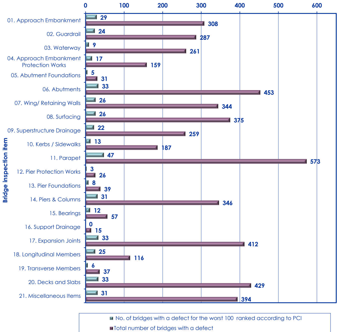
Figure 4-13: Statistics for the defects on bridges
