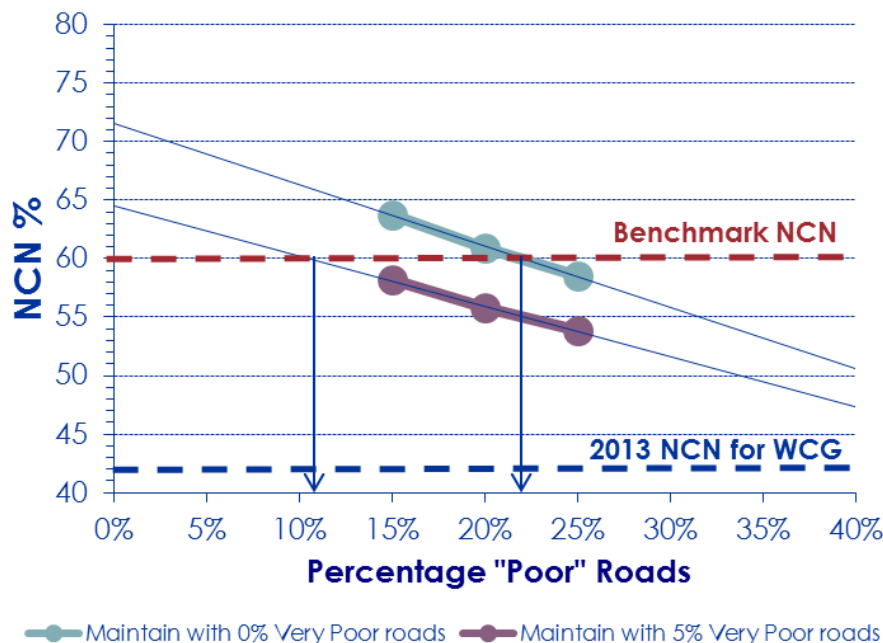
Condition impact graphs for unpaved roads
