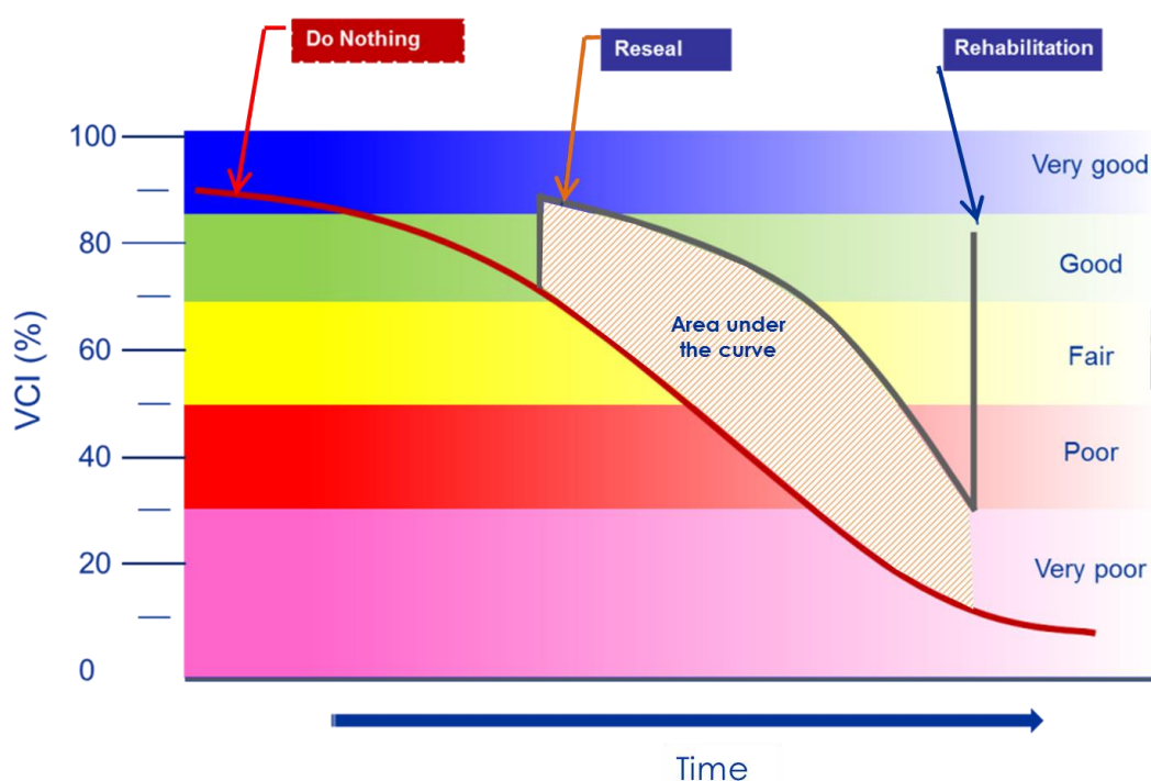
Figure E-1: Illustration of area-under-the-condition curve
