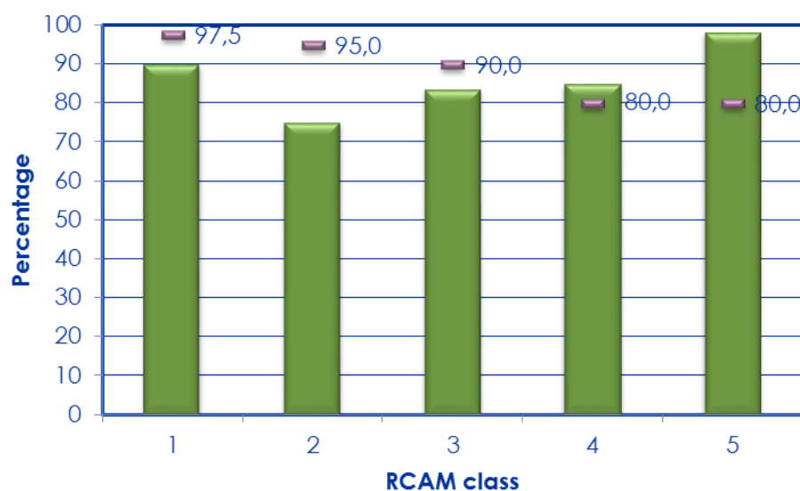
Figure 4-12: High texture exposure per RCAM class compared with preliminary LOS targets in 2015
