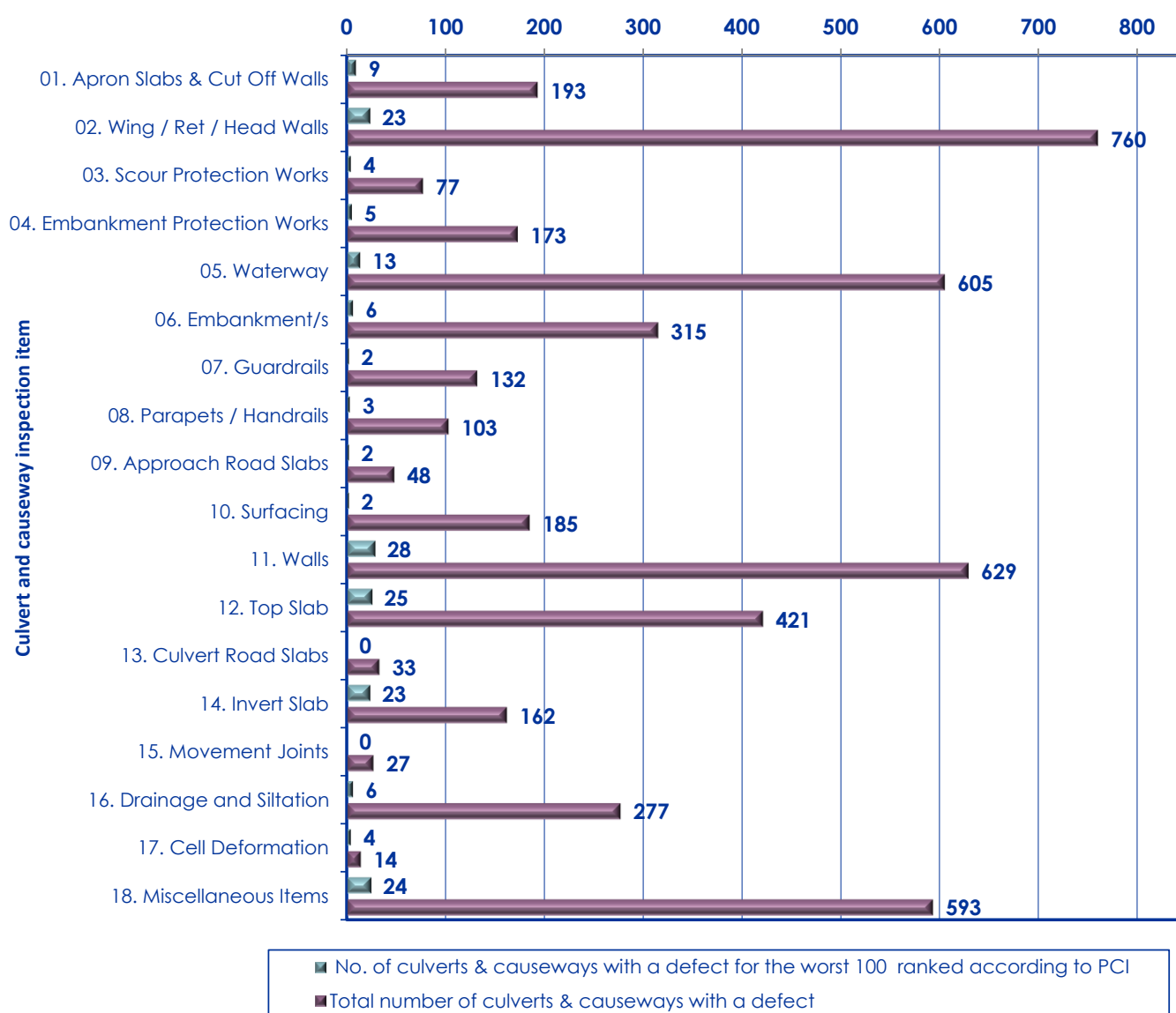
Figure 4-14: Statistics for the defects on culverts and causeways in August 2017
