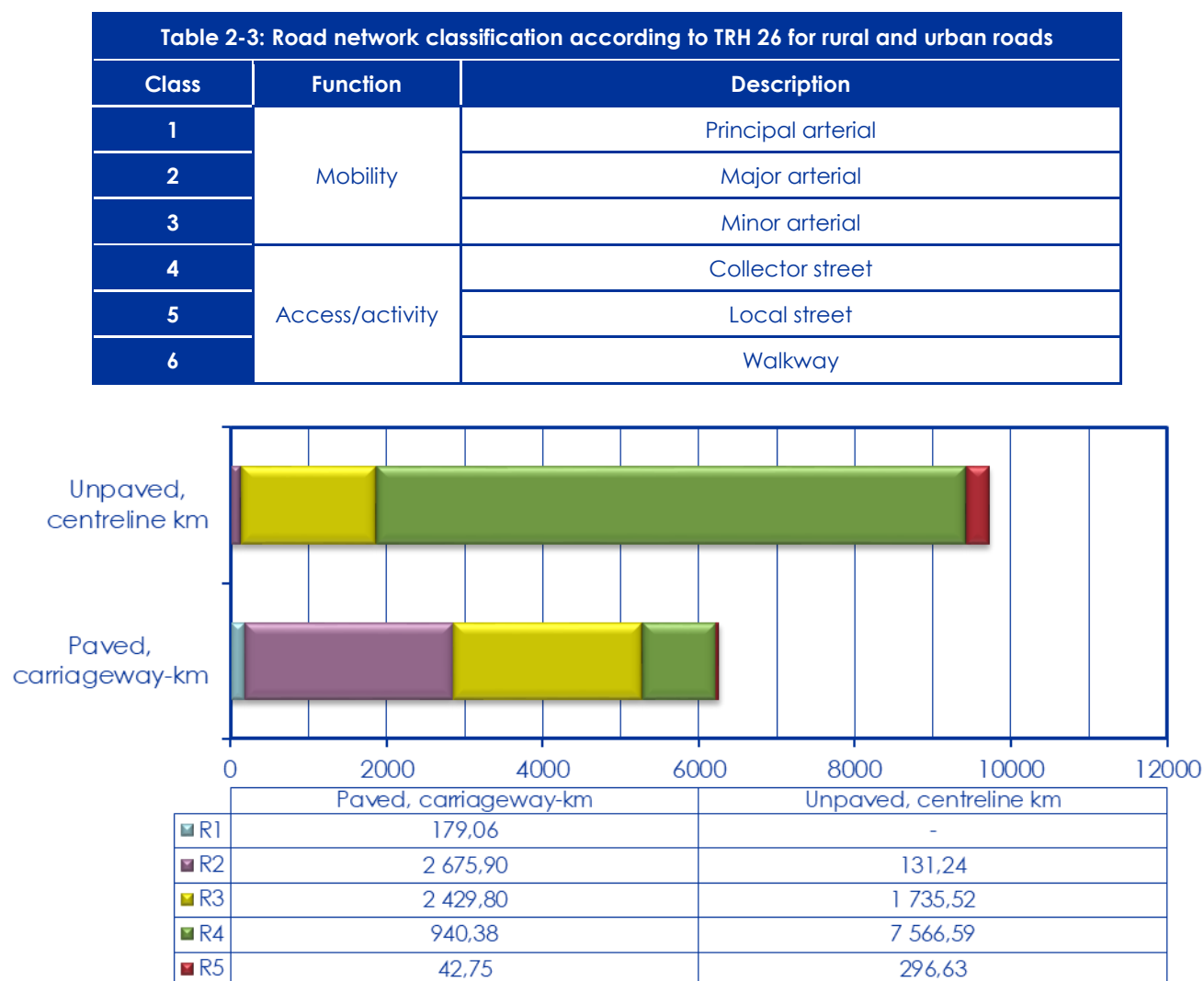
Figure 2-1: The WCG maintained rural road network classification according to TRH 26
