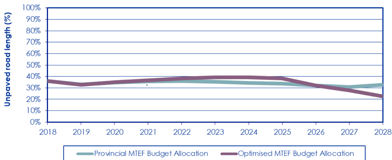
Figure 5-38: Predicted proportion of maintained unpaved roads with possible passability problems where gravel thickness is <50 mm
