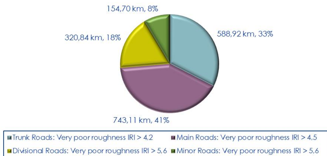
Figure 5-14: Distribution of very poor paved roads according to roughness values in 2016 based on the 2018 length
